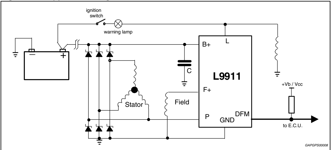
Figure 8. Application diagram
