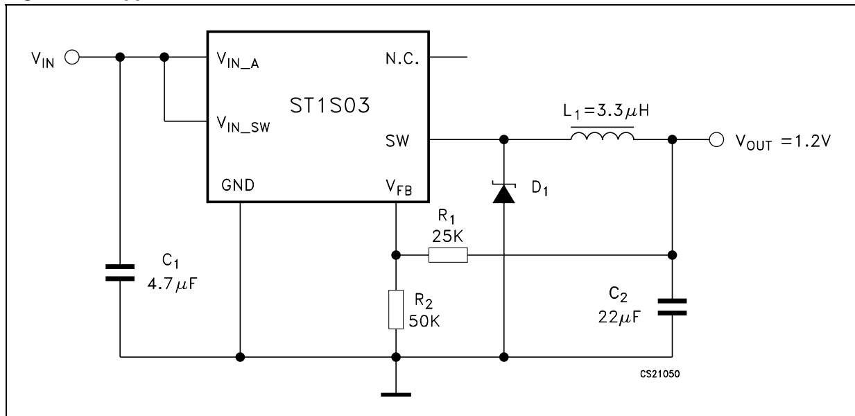
Figure 3. Application circuits
