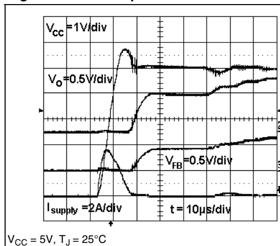
Figure 20. Start-Up transient
