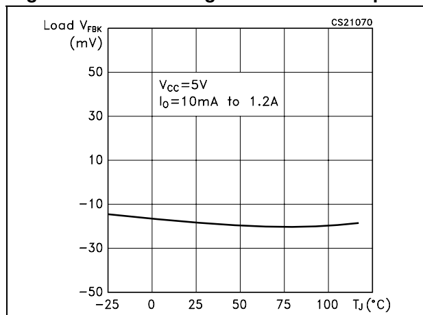
Figure 4. Load voltage feedback vs temp.
