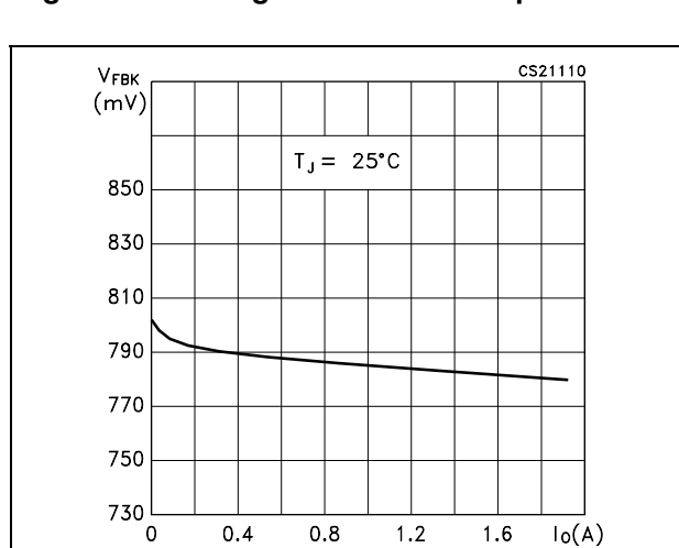
Figure 8. Voltage feedback vs output current
