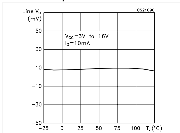
Figure 6. Line output voltage regulation vs temperature
