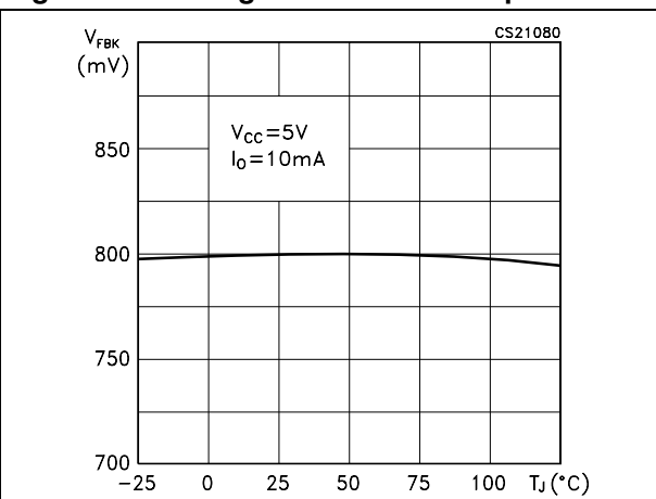
Figure 5. Voltage feedback vs temperature
