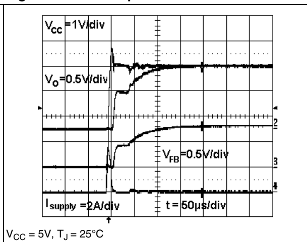
Figure 21. Start-Up transient
