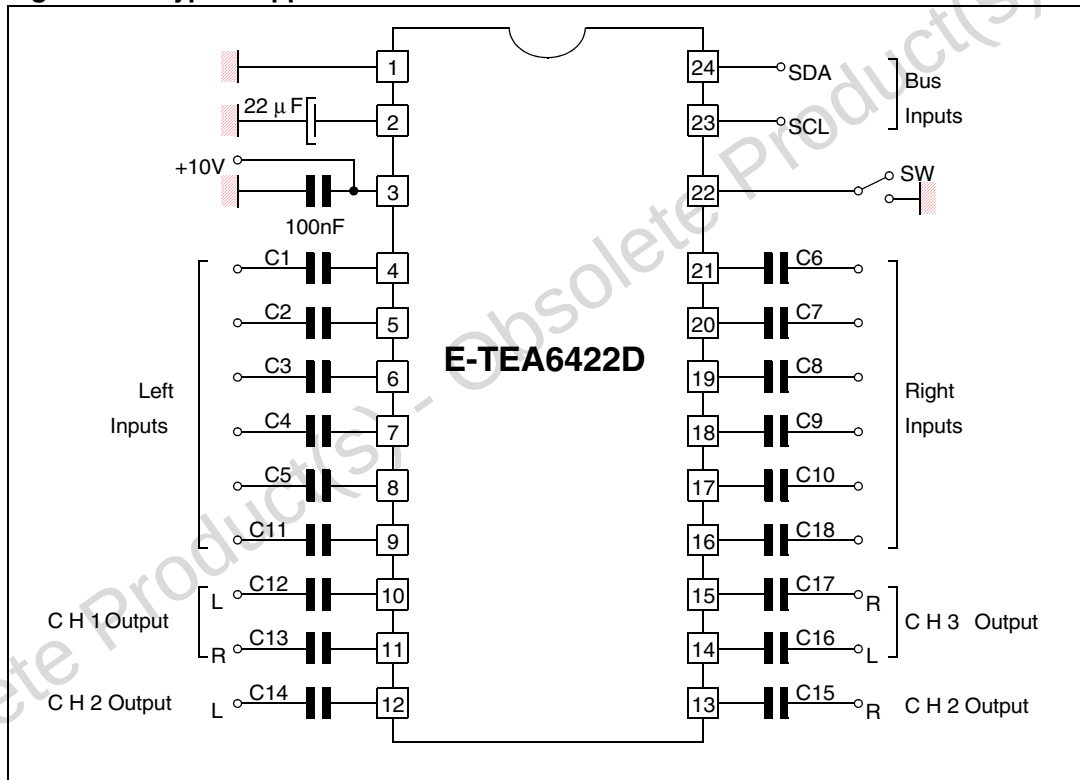
Figure 11. Typical application
