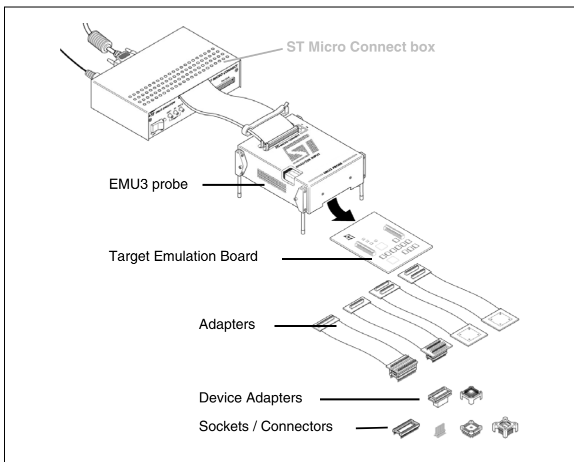
Figure 1: ST7MDTxxx-EMU3 terminology
