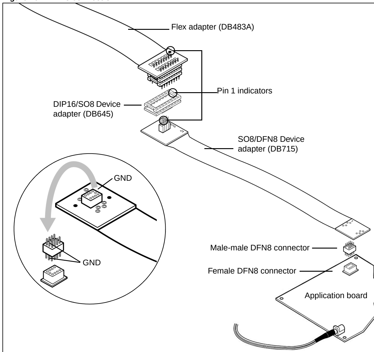
Figure 10. DFN8 connection
