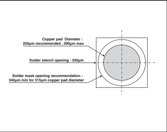
Figure 9. Flip-Chip footprint
