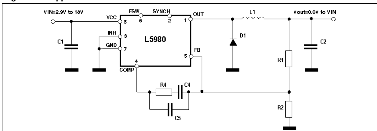
Figure 1. Application circuit
