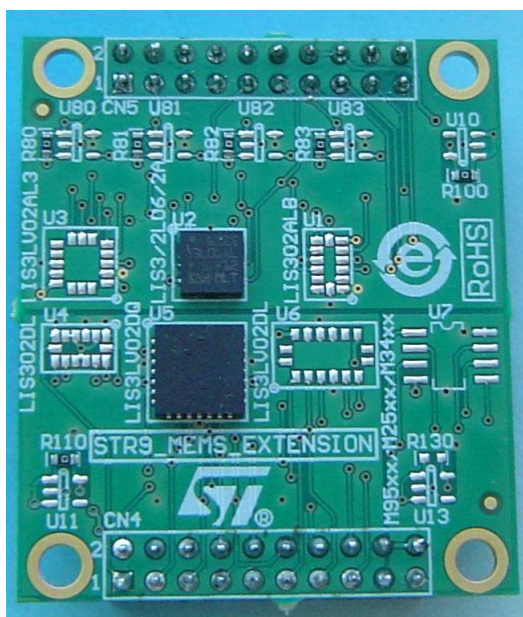
Figure 1. STR9 MEMS extension
