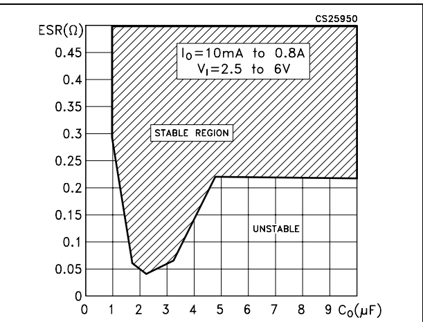
Figure 18. Stability region vs C_O & Low ESR (at 100kHz)
