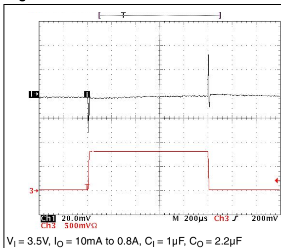
Figure 19. Load transient
