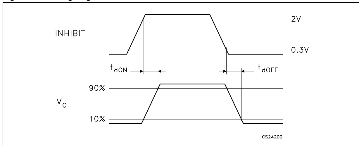
Figure 6. Timing diagram
