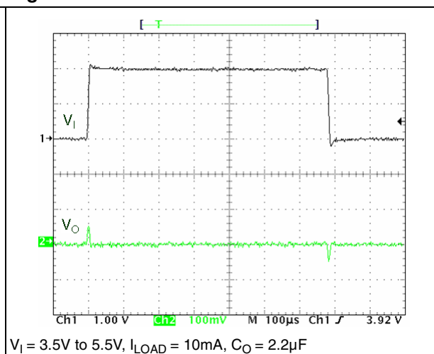
Figure 18. Line transient
