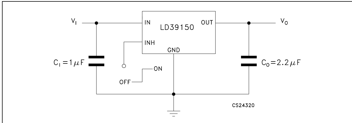
Figure 3. LD39150xx fixed version with inhibit
