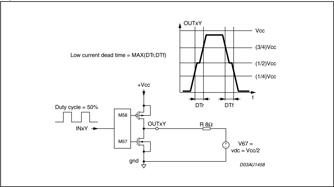
Figure 2. Test circuit
