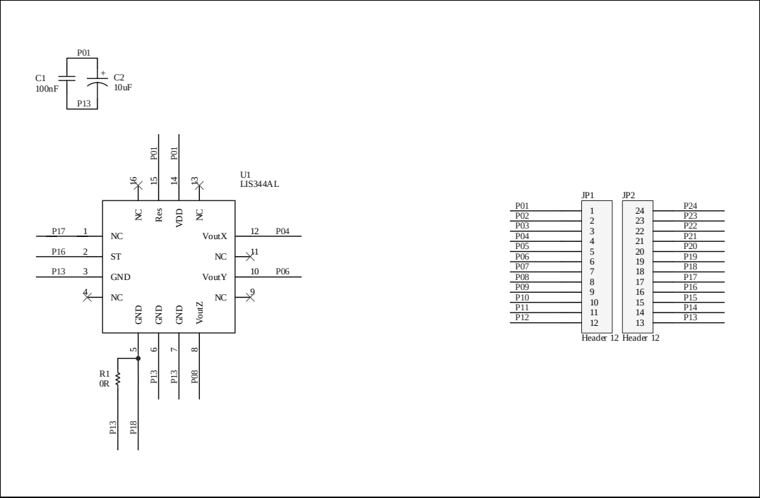
Figure 2. Schematic and connection diagram for the STEVAL-MKI017V1
