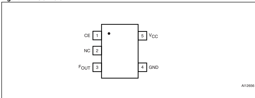
Figure 1. SOT23-5L
