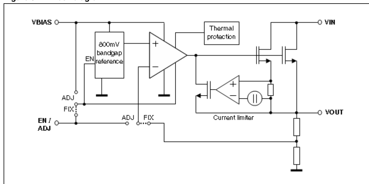
Figure 6. Block diagram
