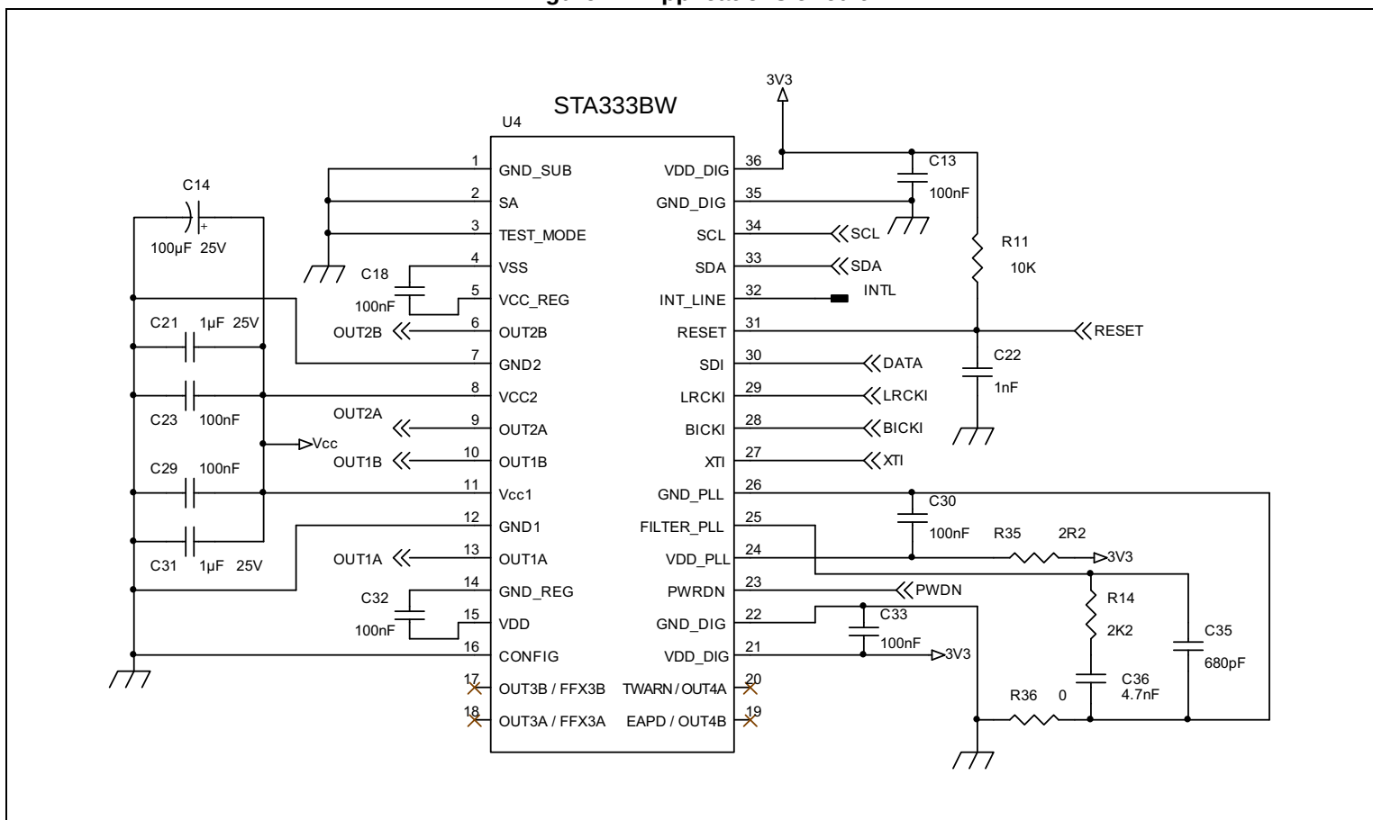
Figure 21. Applications circuit
