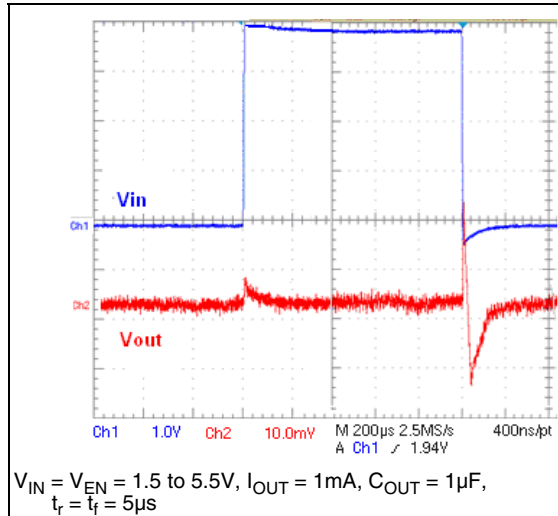
Figure 12. Line transient
