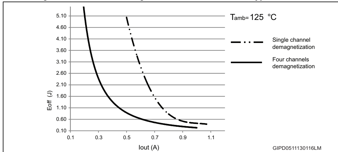
Figure 14. Maximum demagnetization vs. load current, typical values
