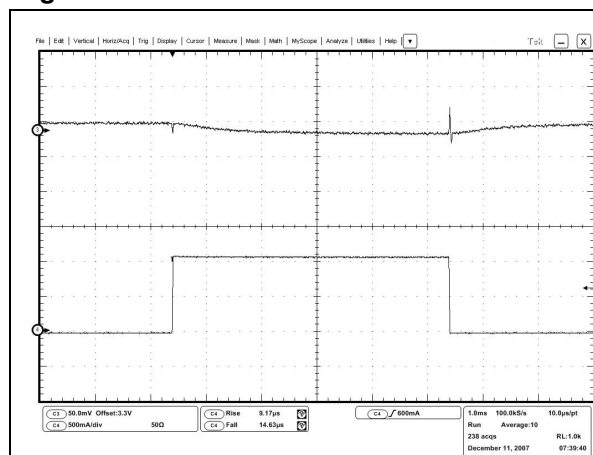
Figure 20. Load transient
