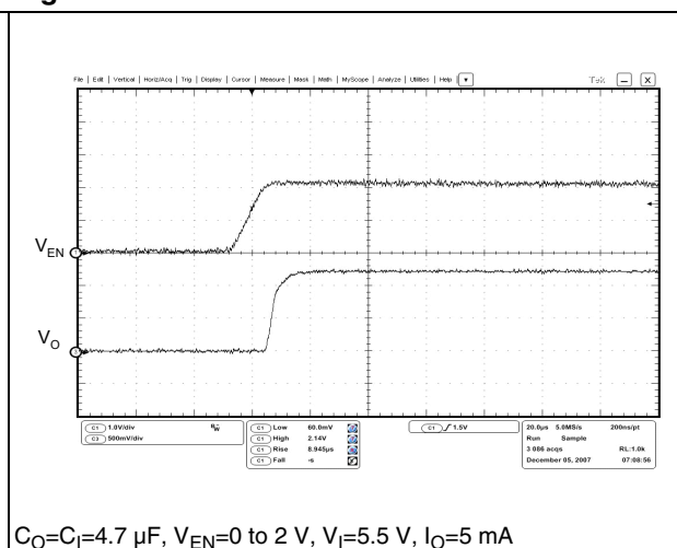
Figure 23. Enable transient
