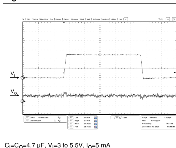
Figure 22. Line transient
