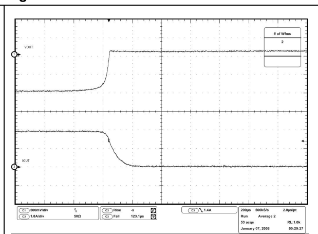
Figure 21. Short-circuit removal transient
