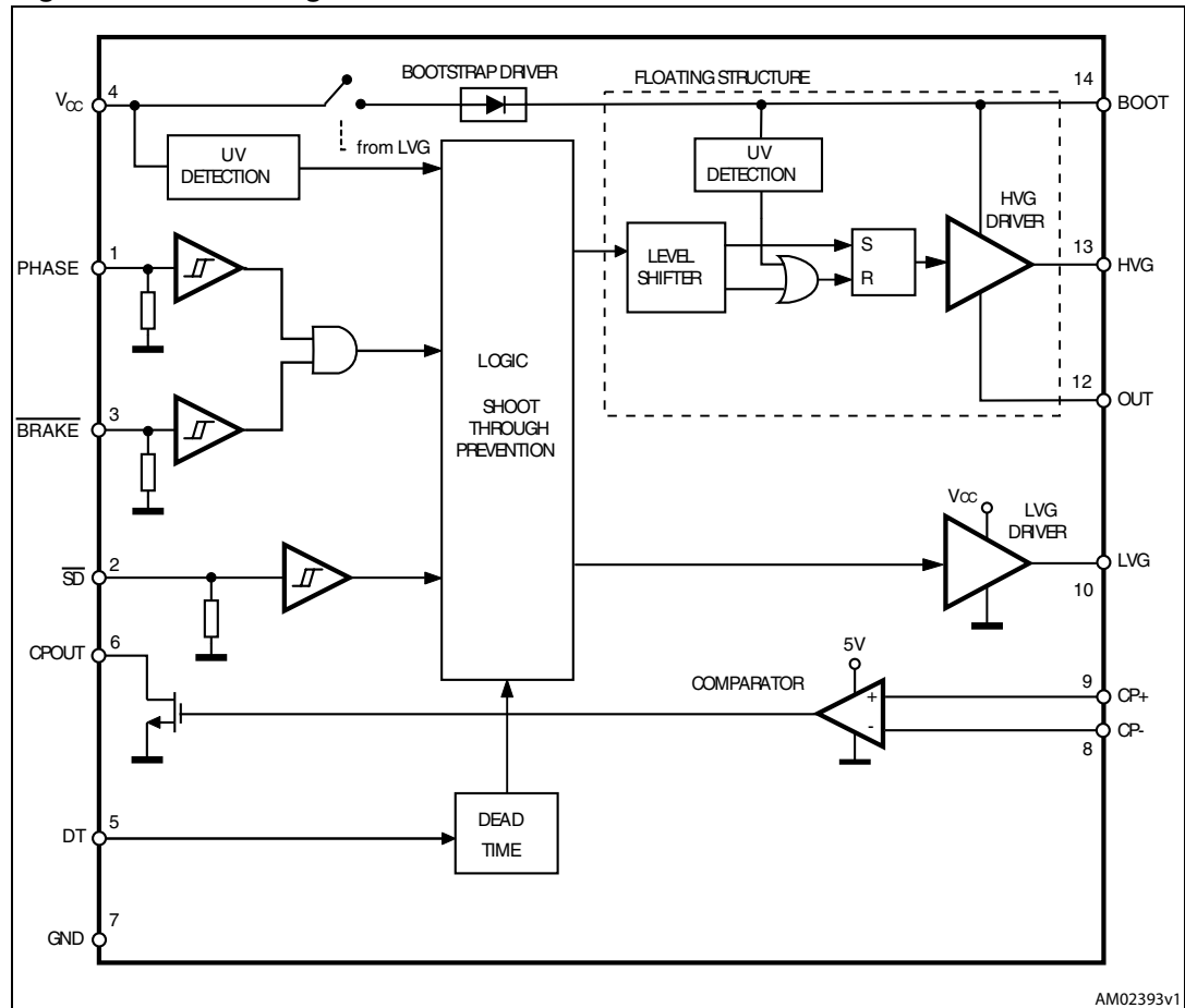
Figure 1. Block diagram
