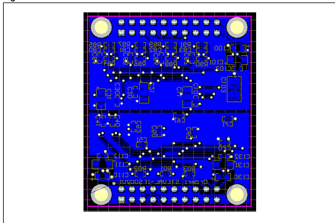
Figure 11. Bottom view
