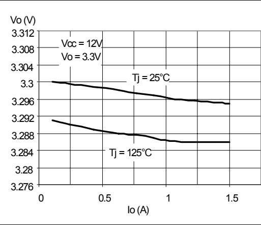
Figure 27. Load regulation
