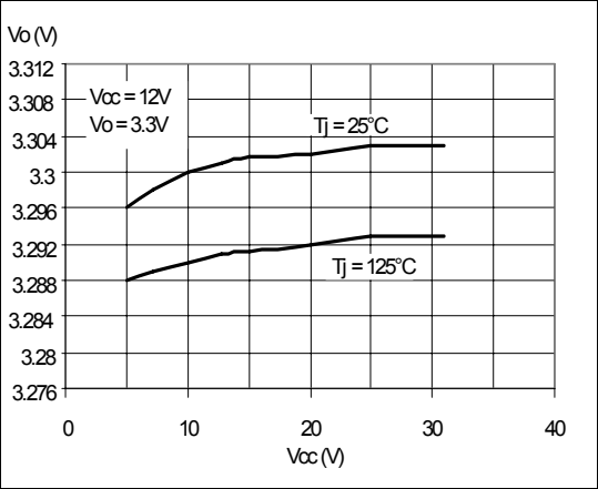
Figure 28. Line regulation
