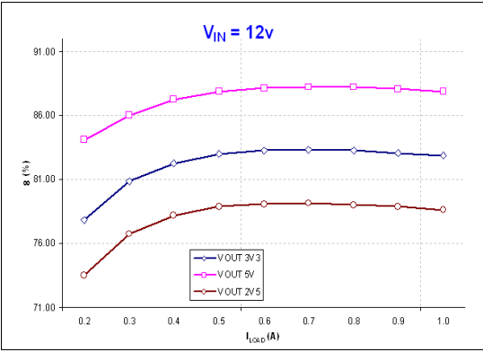
Figure 33. Efficiency vs output current
