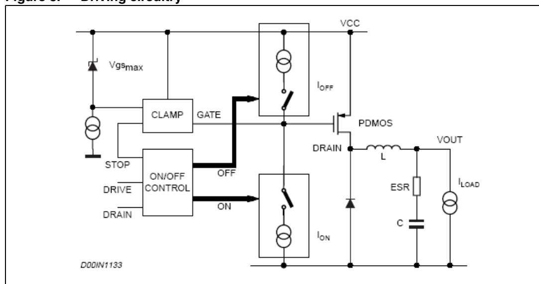
Figure 8. Driving circuitry
