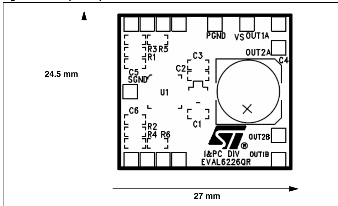
Figure 4. Component placement
