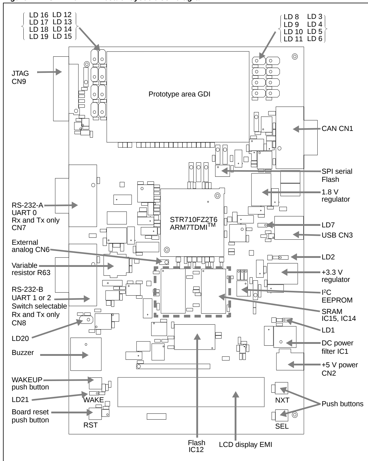
Figure 2. STR710-EVAL board layout block diagram
