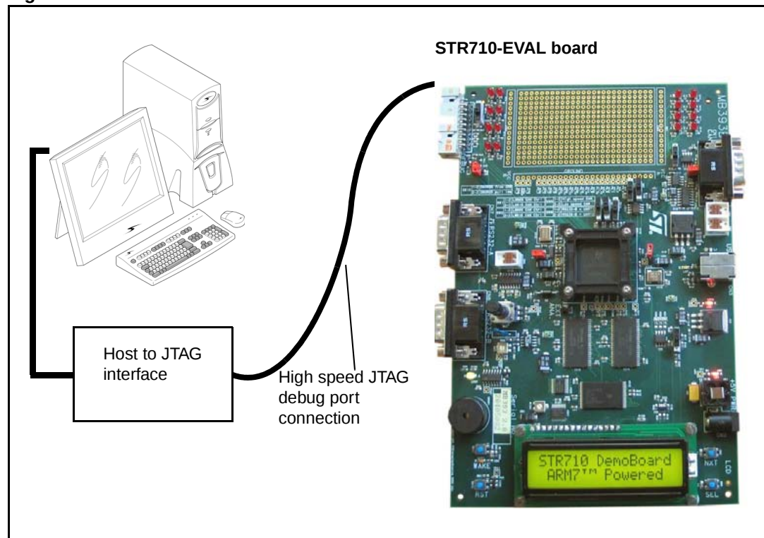
Figure 1. STR710-EVAL board
