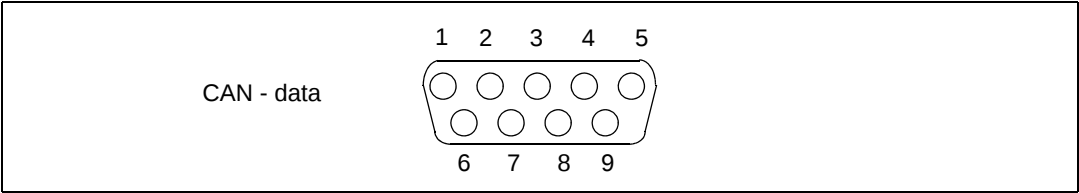
Figure 8. CAN connector 9 pin male D-type: CN1
