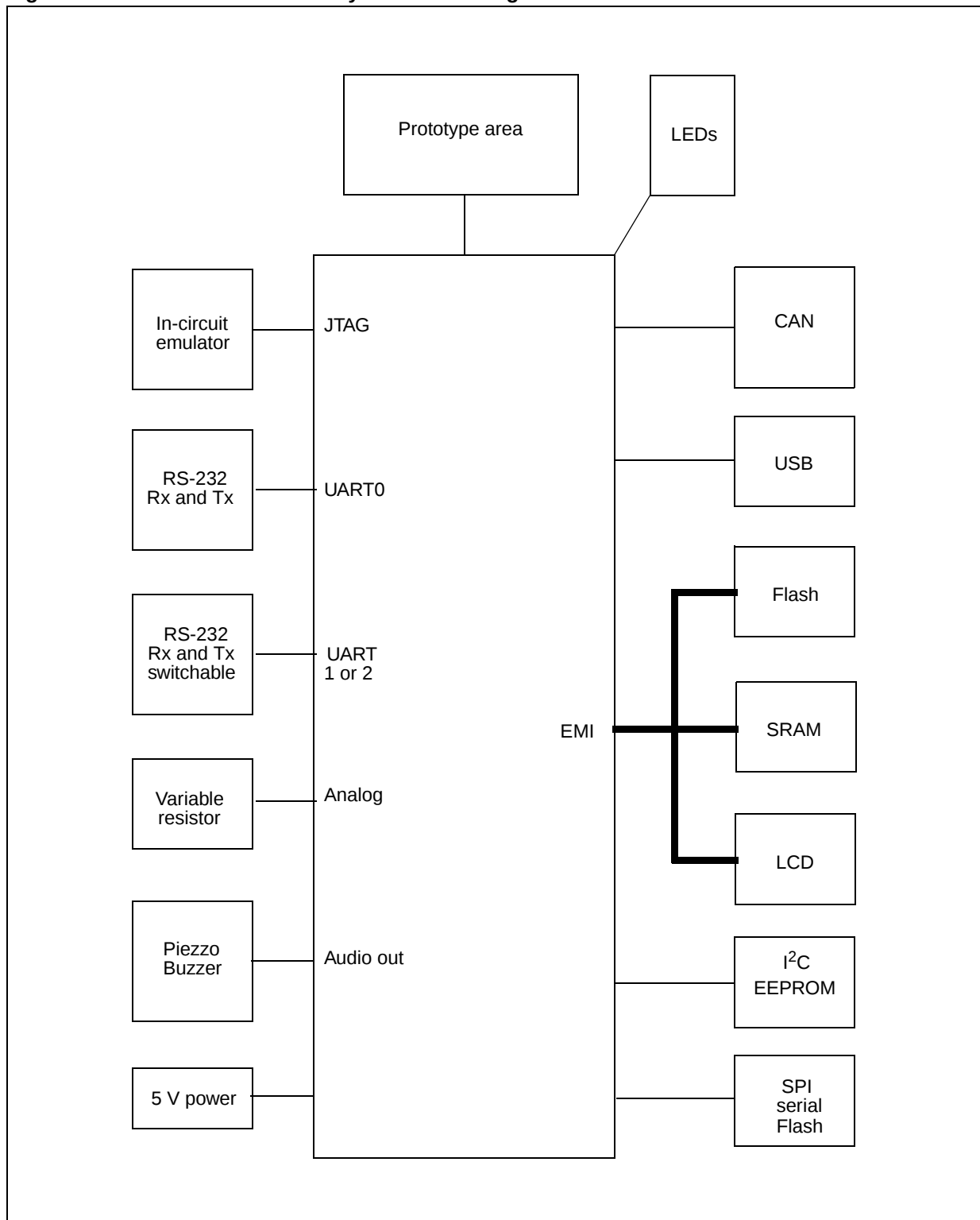
Figure 3. STR710-EVAL board system block diagram
