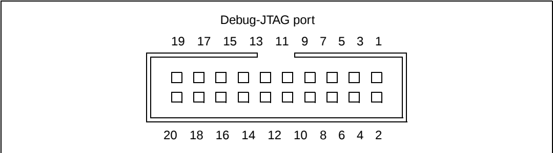
Figure 11. JTAG standard interface: CN9
