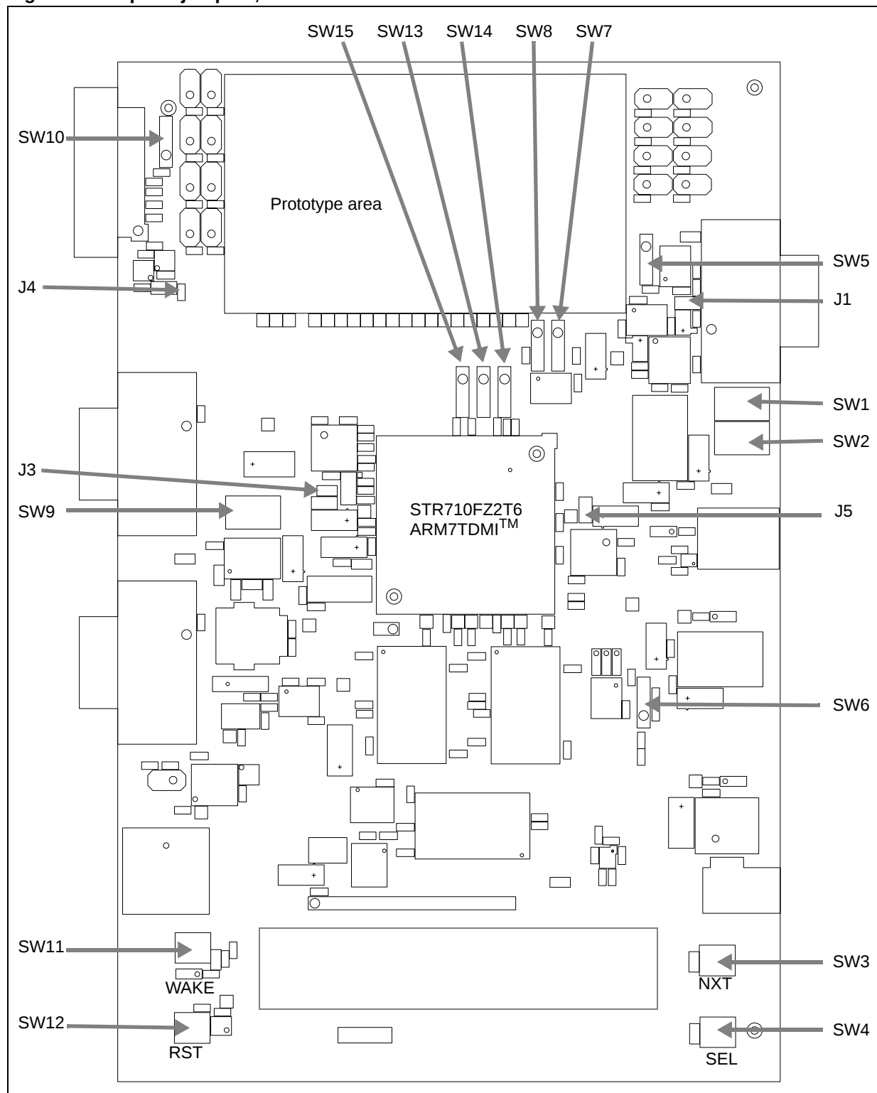
Figure 4. Option jumpers, resistors and switches
