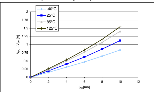
Figure 32. Typ. V_{DD} - V_{OH} @ V_{DD} = 5.0 V (high sink ports)
