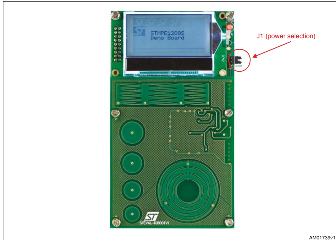
Figure 7. STMPE1208S capacitive touch sensor demonstration board
