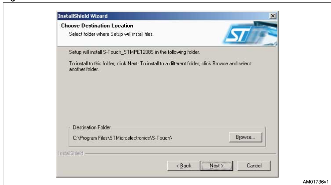
Figure 4. Destination folder
