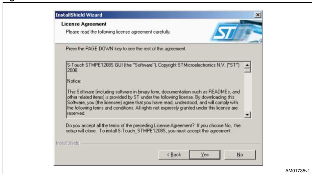
Figure 3. License window
