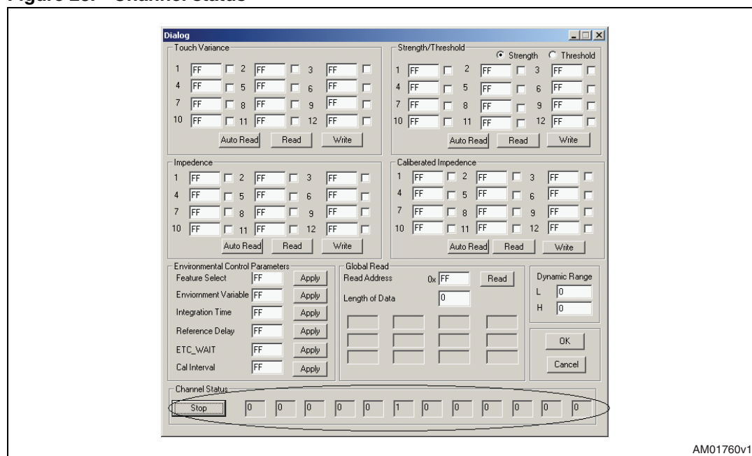
Figure 28. Channel status
