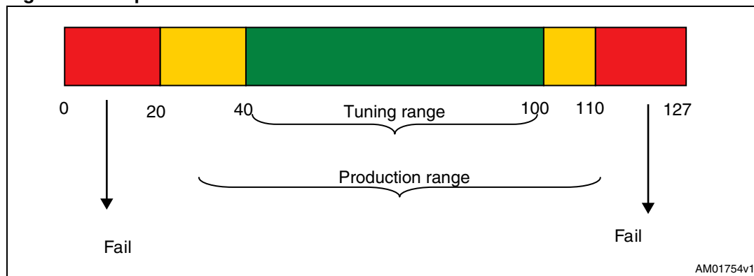
Figure 22. Impedance values
