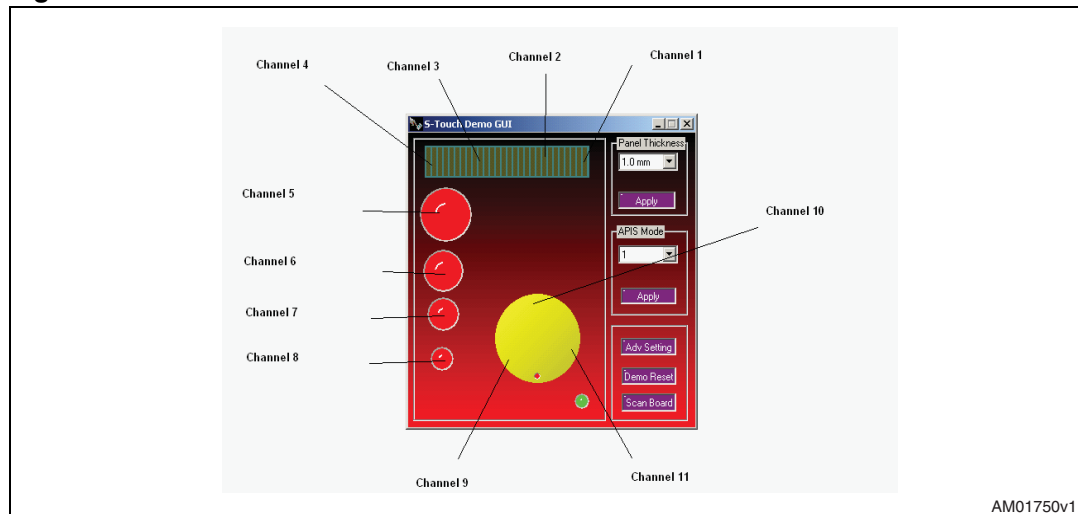
Figure 18. S-Touch™ GUI
