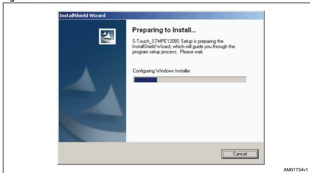
Figure 2. Installation window
