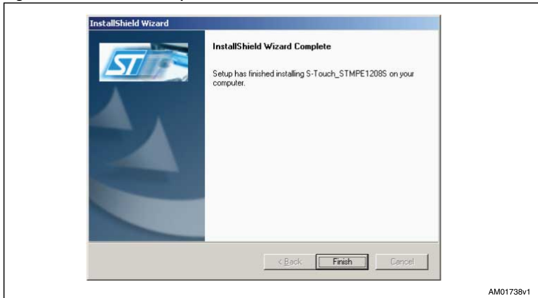
Figure 6. Installation complete
