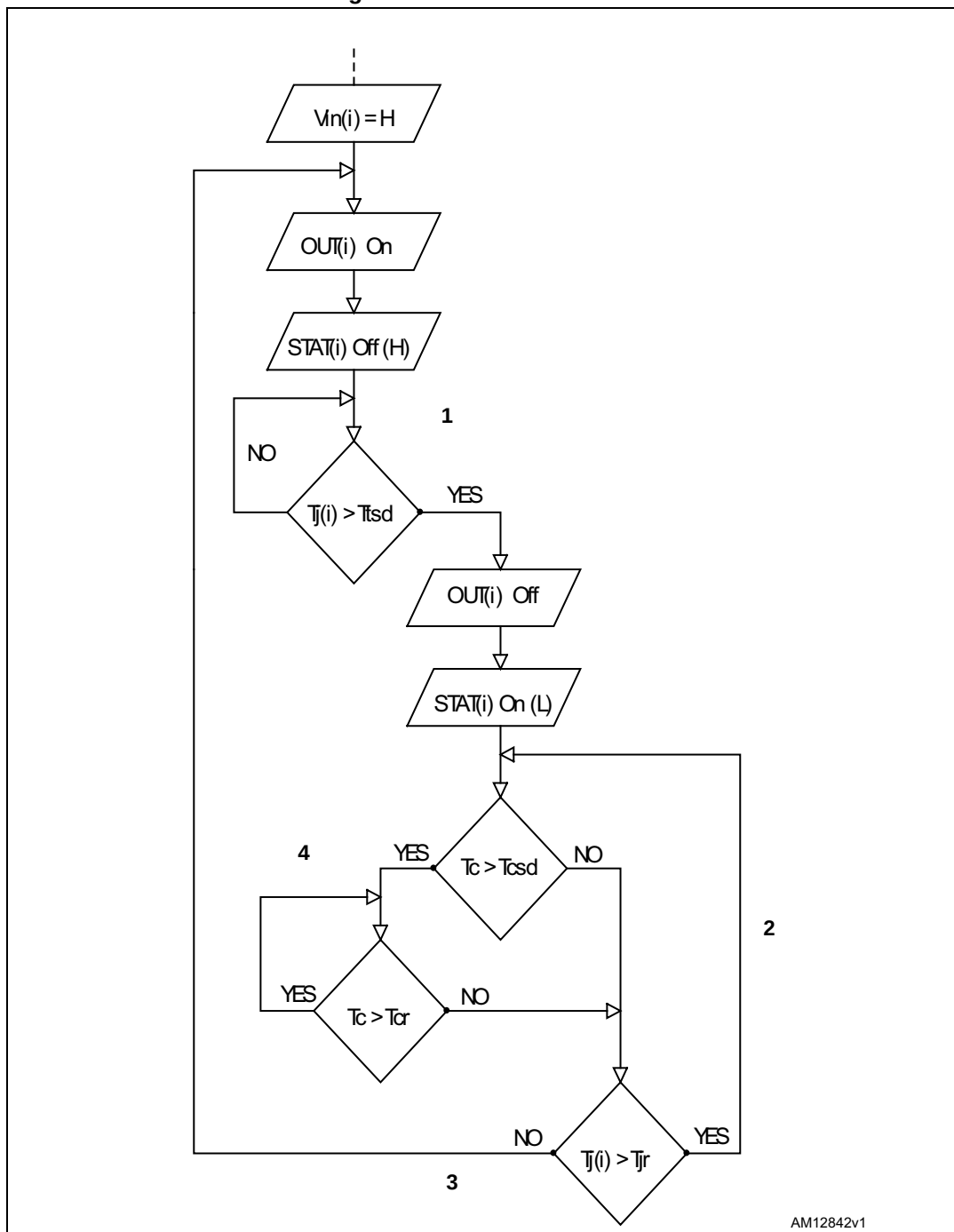
Figure 14. Thermal behavior
