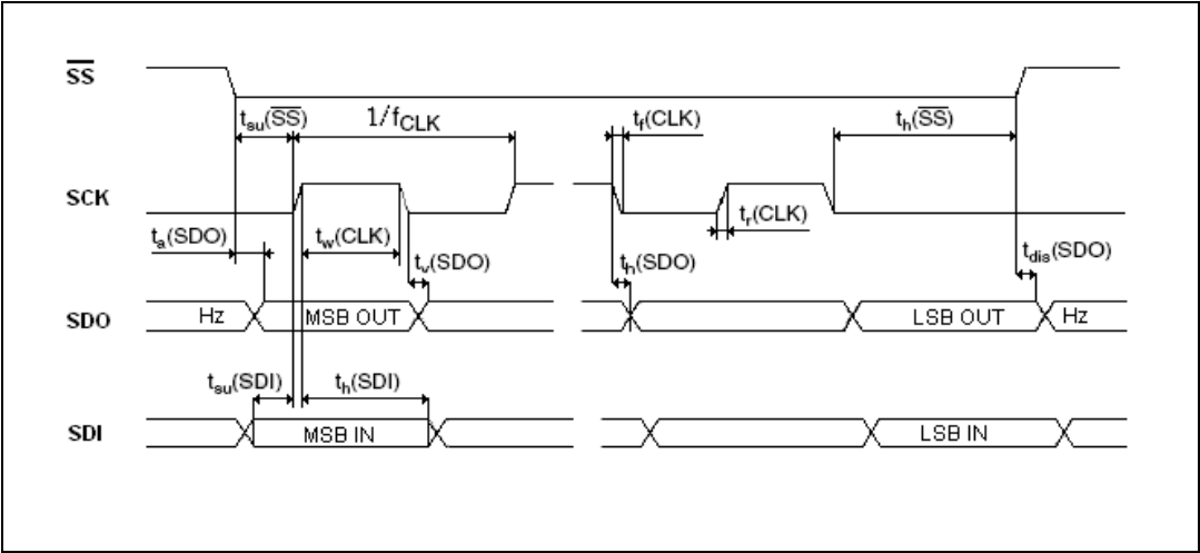
Figure 15. Serial timing
