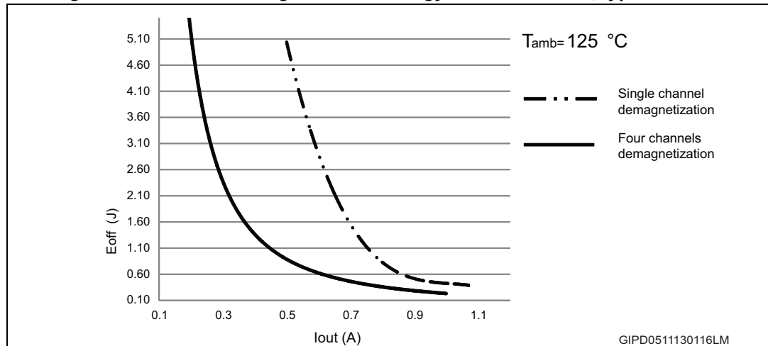
Figure 4. Maximum demagnetization energy vs. load current, typical values
