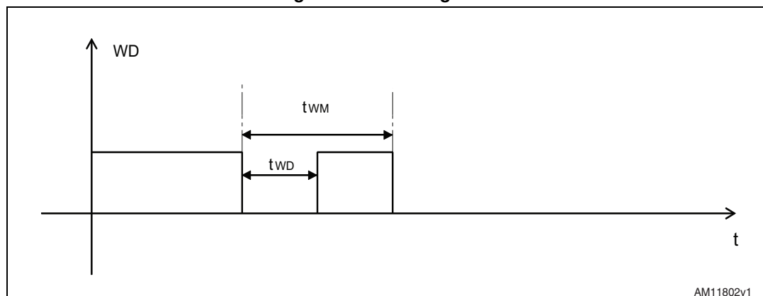
Figure 8. Watchdog reset
