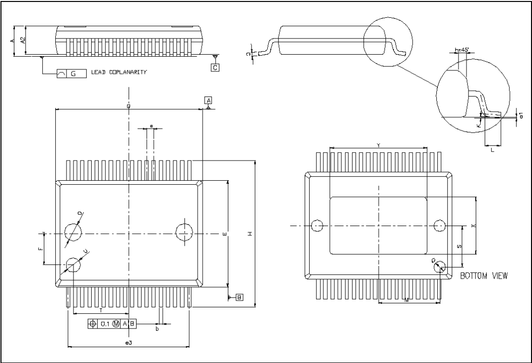
Figure 19. PowerSSO-36 tube shipment (no suffix)
