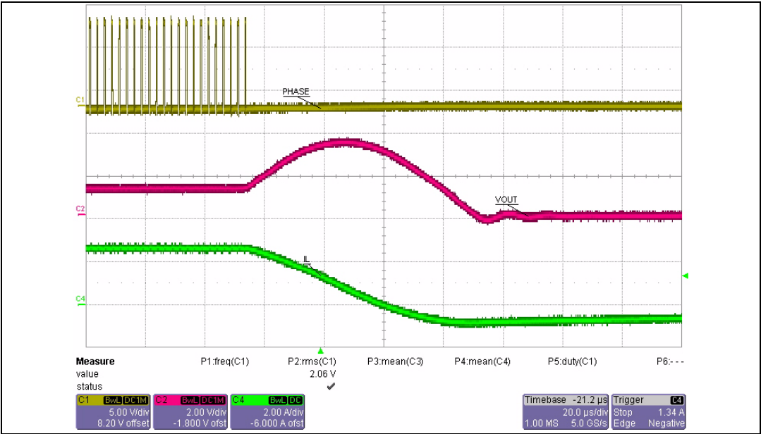
Figure 10. OVP latched
