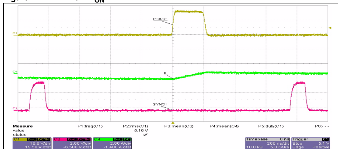
Figure 12. minimum T_{ON}
