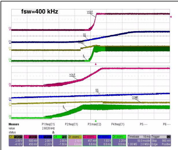
Figure 40. Soft-start
