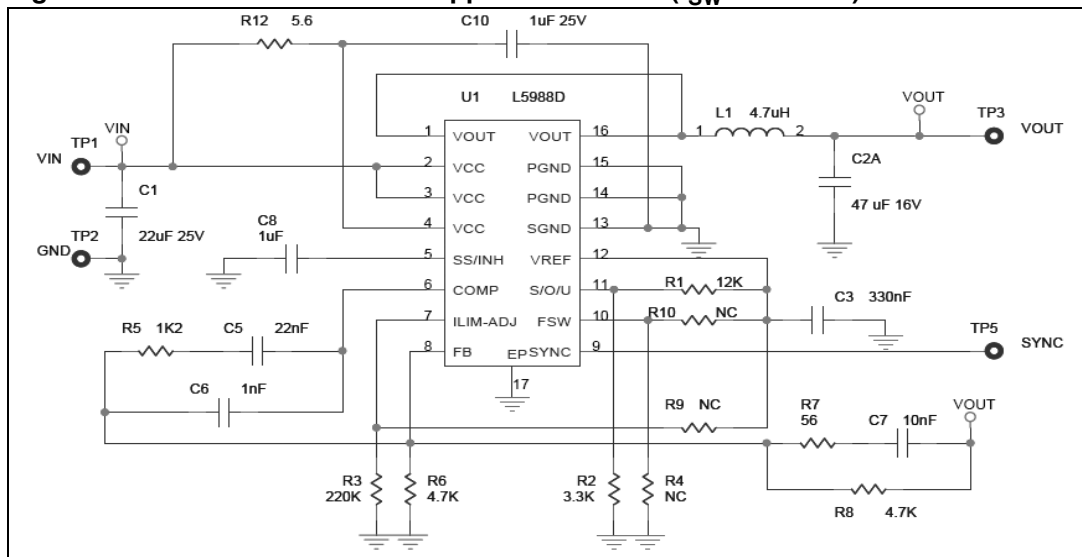
Figure 26. Demonstration board application circuit ( f_{SW} = 400 kHz)
