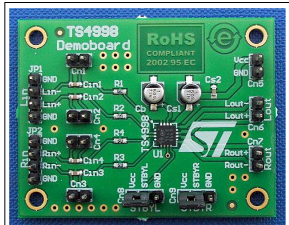
STEVAL-CCA008V1
