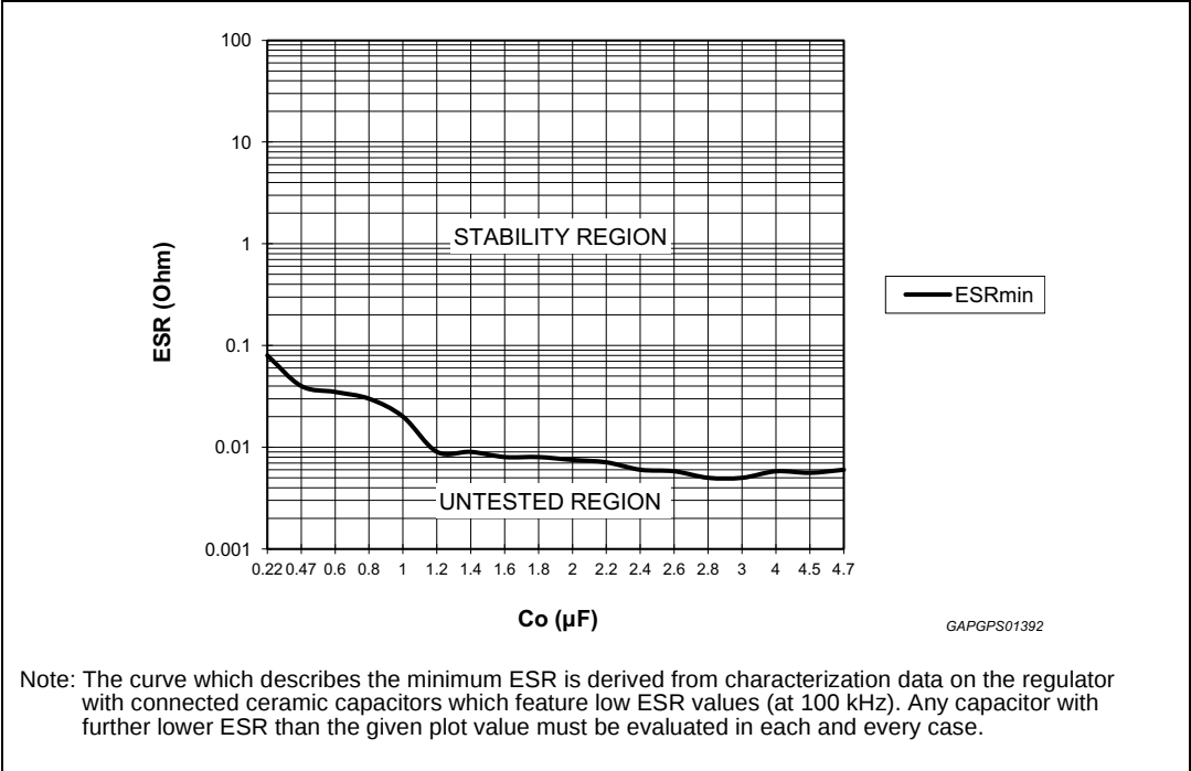
Figure 25. Stability region
