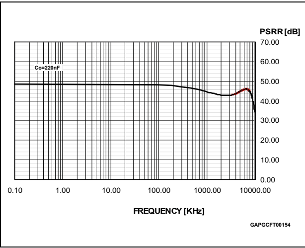
Figure 23. PSRR
