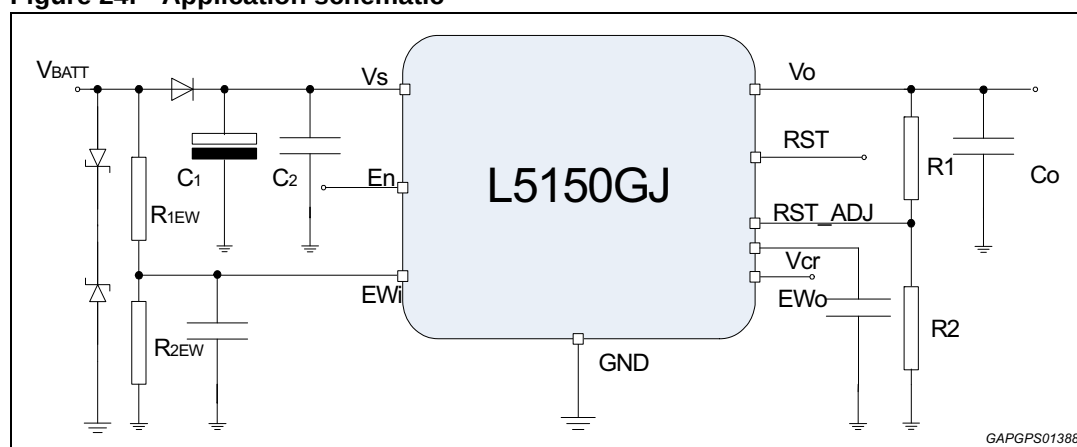
Figure 24. Application schematic
