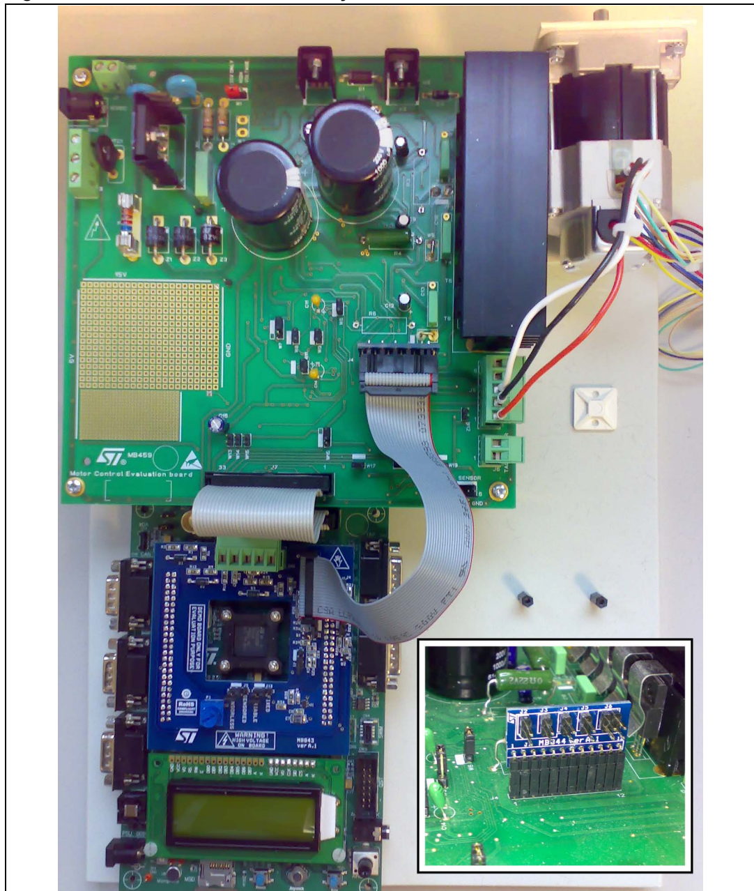
Figure 2. STM8/128-MCKIT assembly
