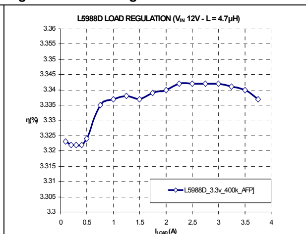
Figure 36. Load regulation
