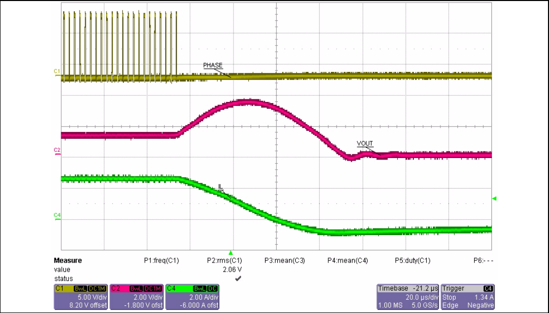
Figure 9. OVP latched
