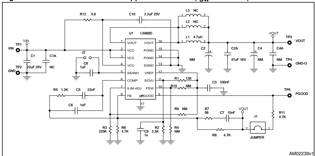
Figure 25. Demonstration board application circuit ( f_{SW} = 400 \text{ kHz} )
