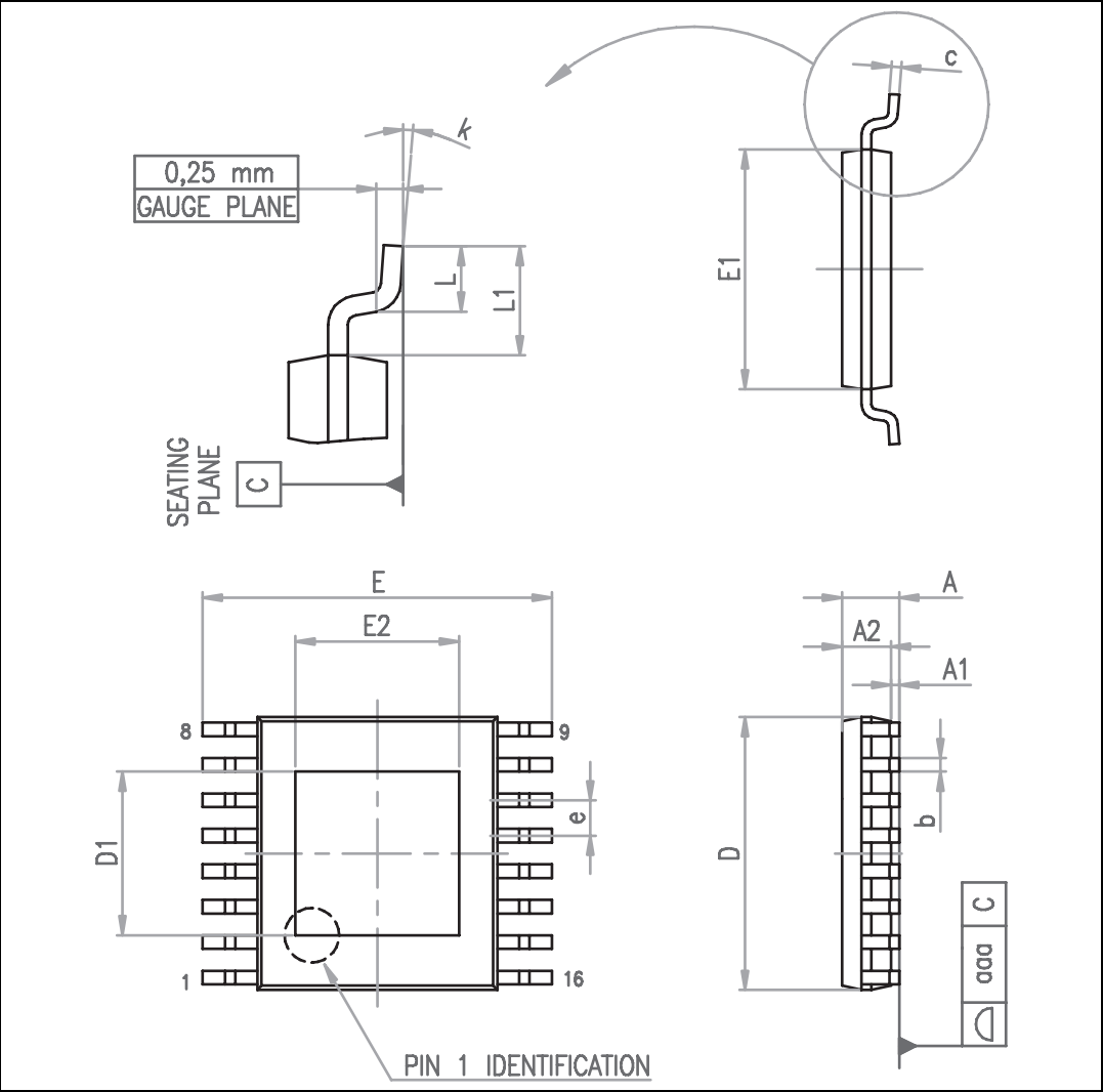
Figure 40. Mechanical drawing
