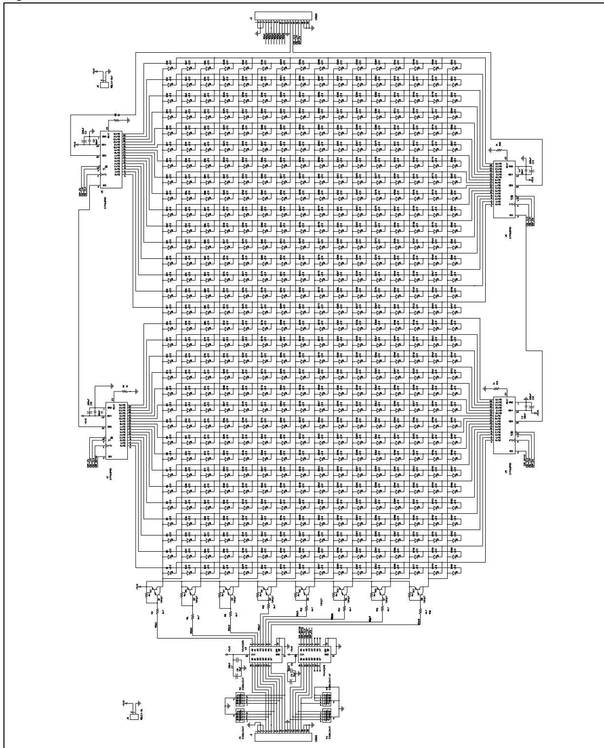
Figure 1. Circuit schematic
