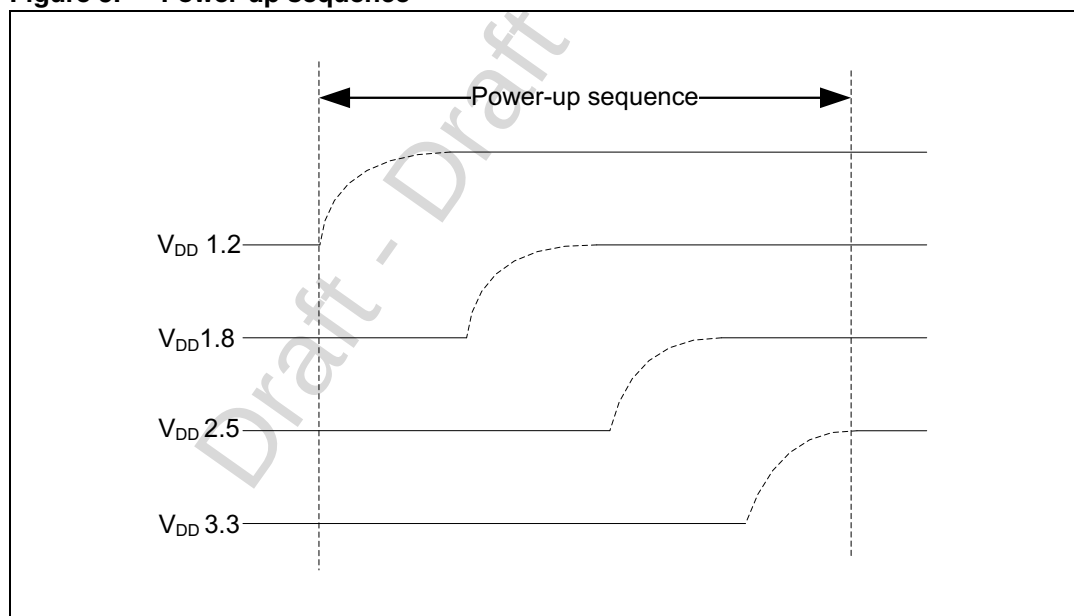
Figure 5. Power-up sequence
