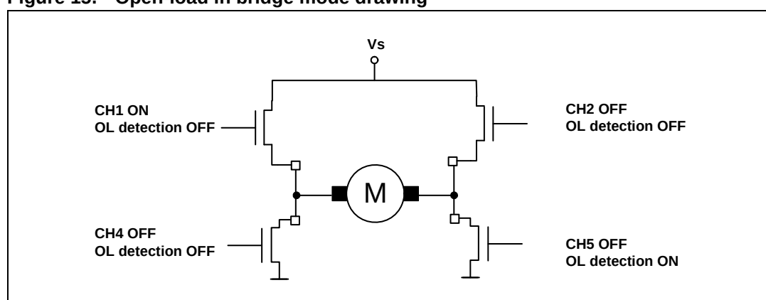
Figure 15. Open-load in bridge mode drawing
