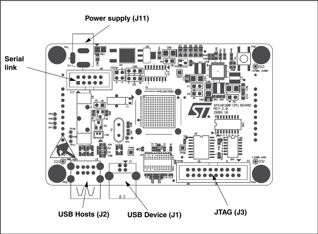
Figure 24. CPU board layout (top view)
