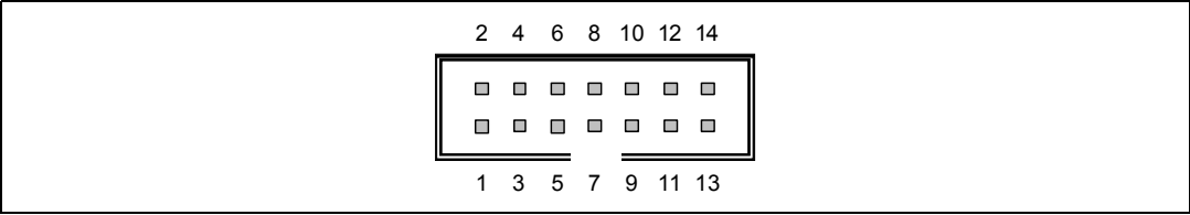
Figure 11. Digital output parallel connector (CN6) pinout
