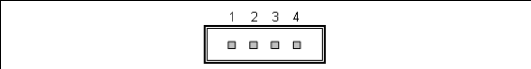
Figure 16. RS-485 header connector CN12 pinout
