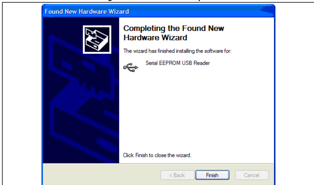
Figure 36. Installation complete
