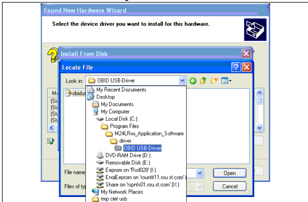
Figure 16. Locate file
