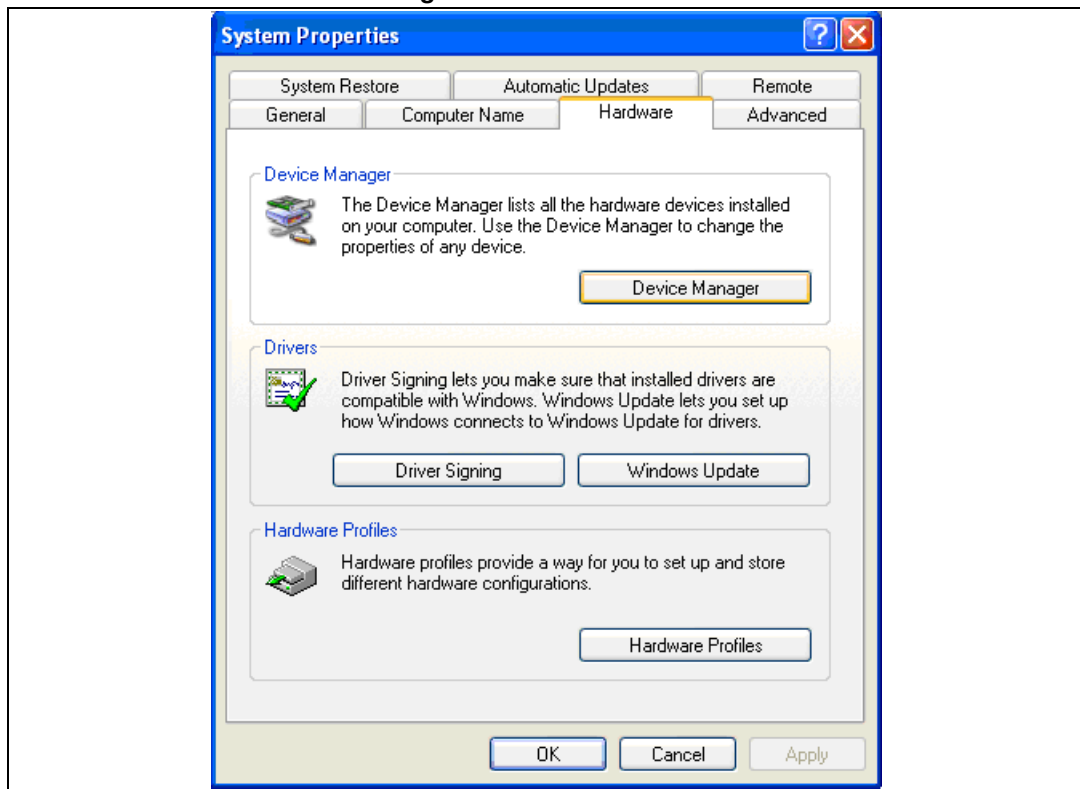
Figure 24. Hardware tab
