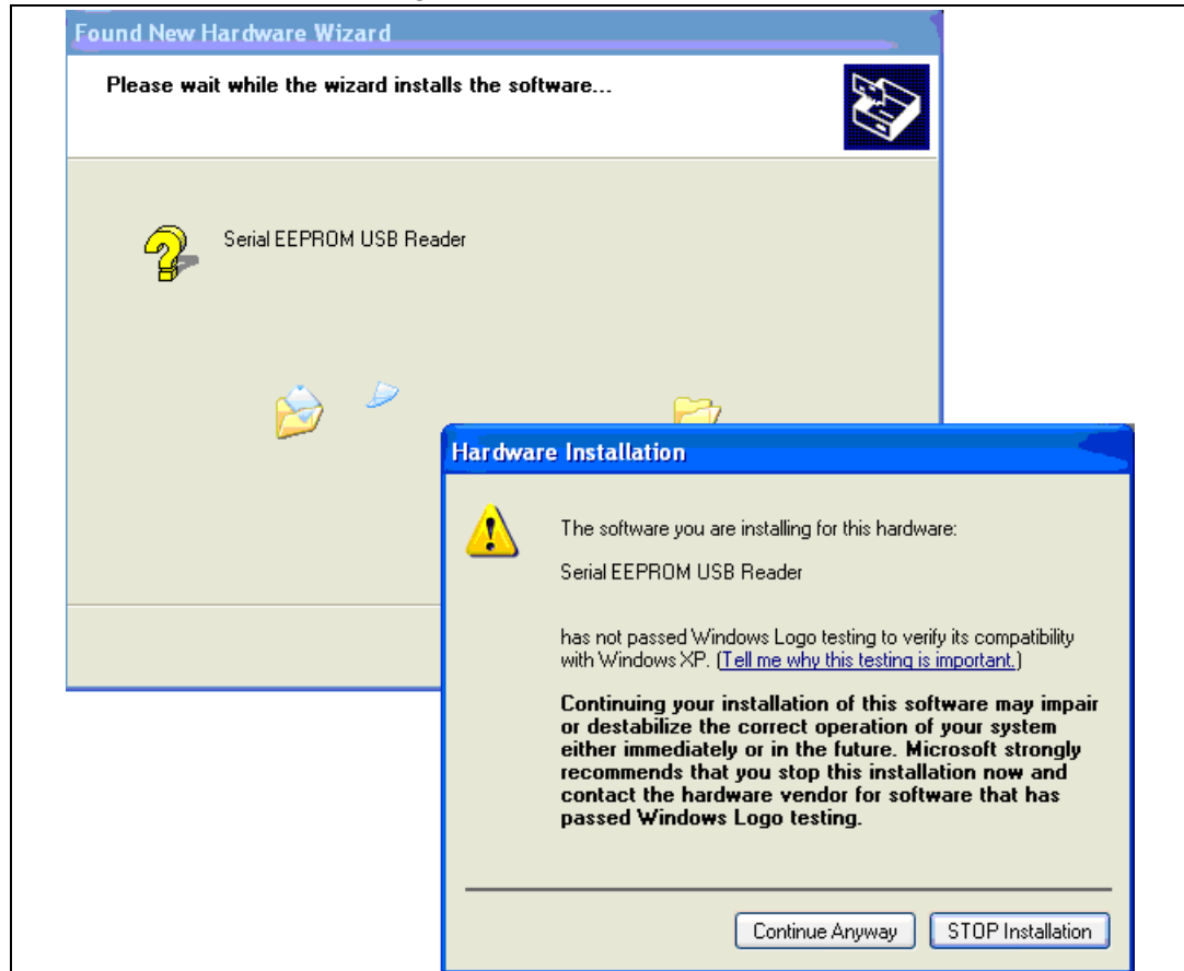
Figure 35. Software installation
