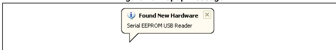
Figure 26. Popup message
