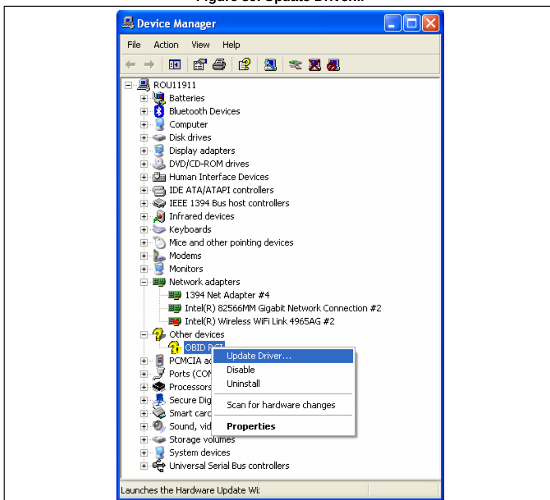
Figure 39. Update Driver...
