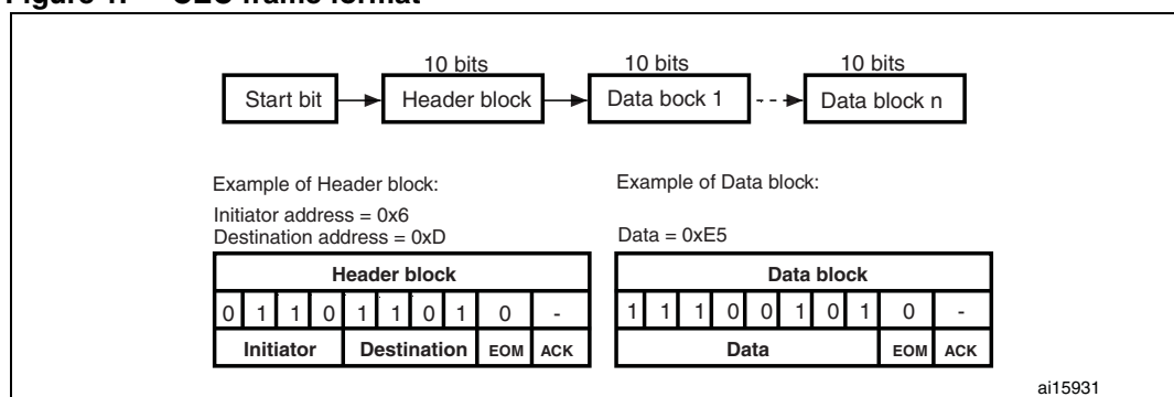
Figure 1. CEC frame format
