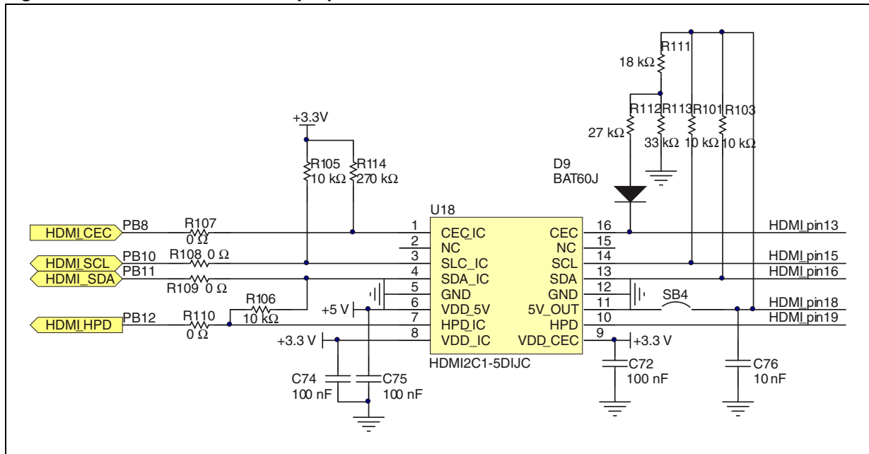
Figure 12. Electrical schematic proposal for STM32100B-EVAL
