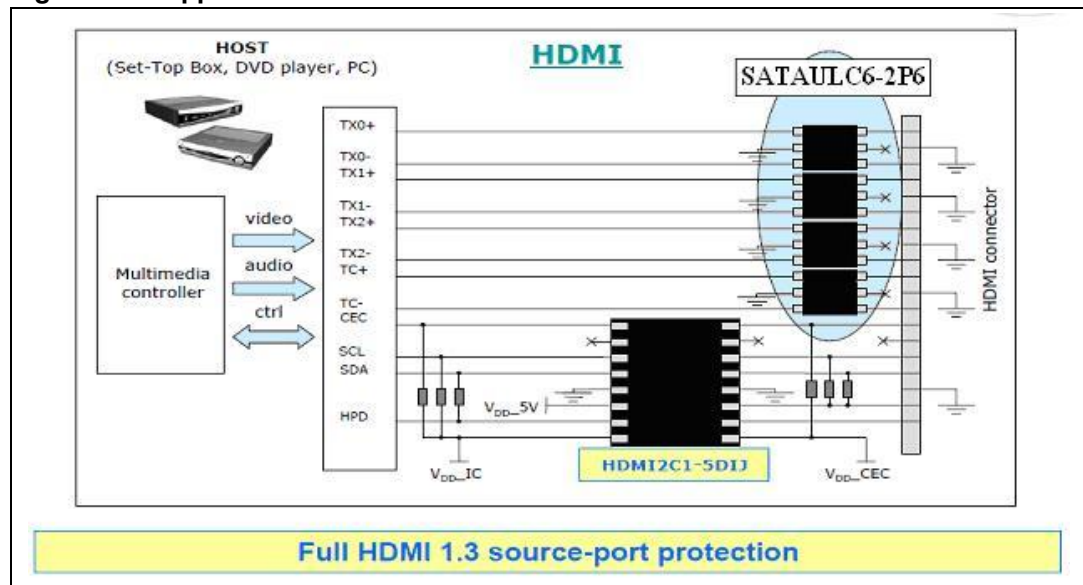
Figure 11. Application schematic
