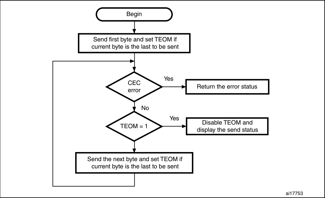
Figure 23. Send flowchart
