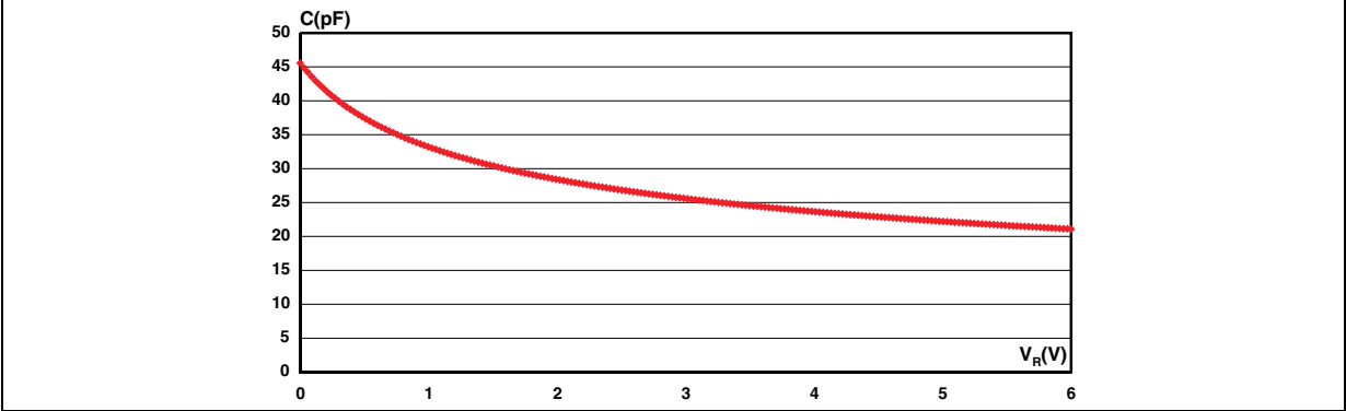
Figure 11. Line capacitance versus applied voltage
