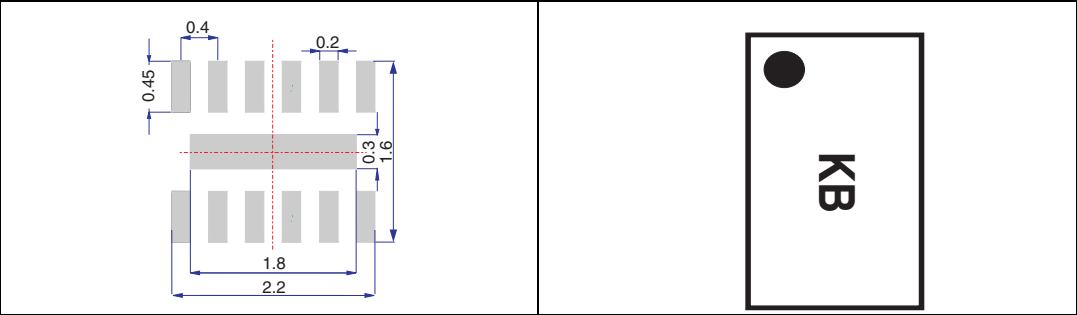
Figure 13. Footprint recommendations
