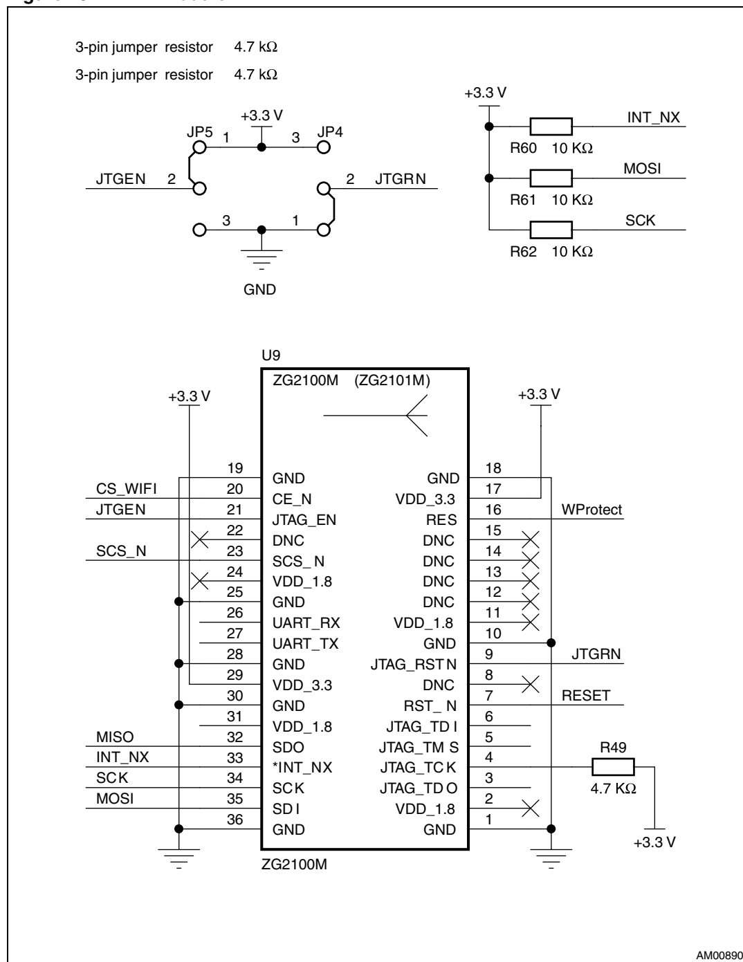
Figure 23. Wi-Fi module-2
