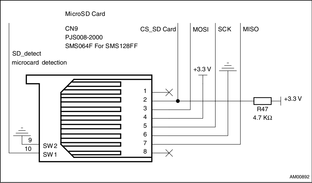
Figure 24. MicroSD Card
