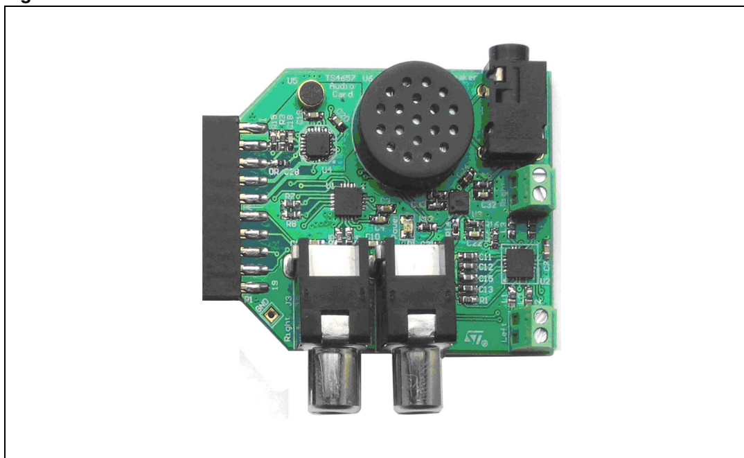
Figure 2. STEVAL-CCA021V1
