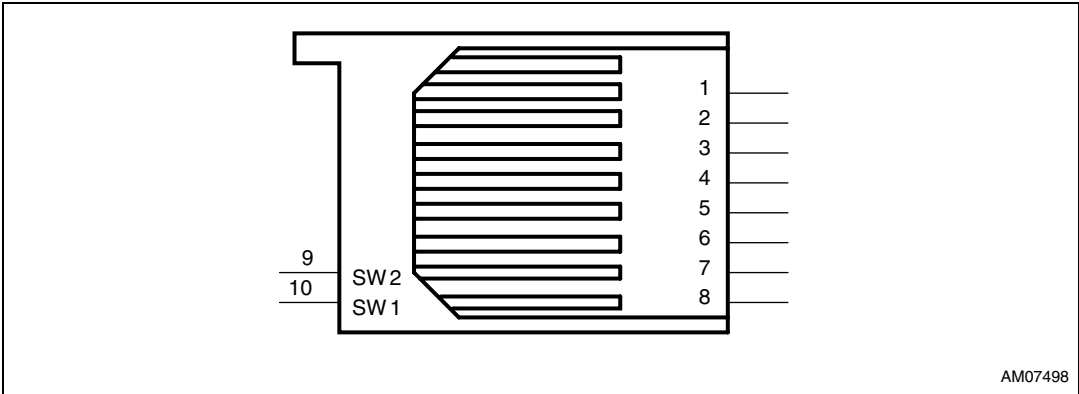
Figure 13. MicroSD Card connector CN9
