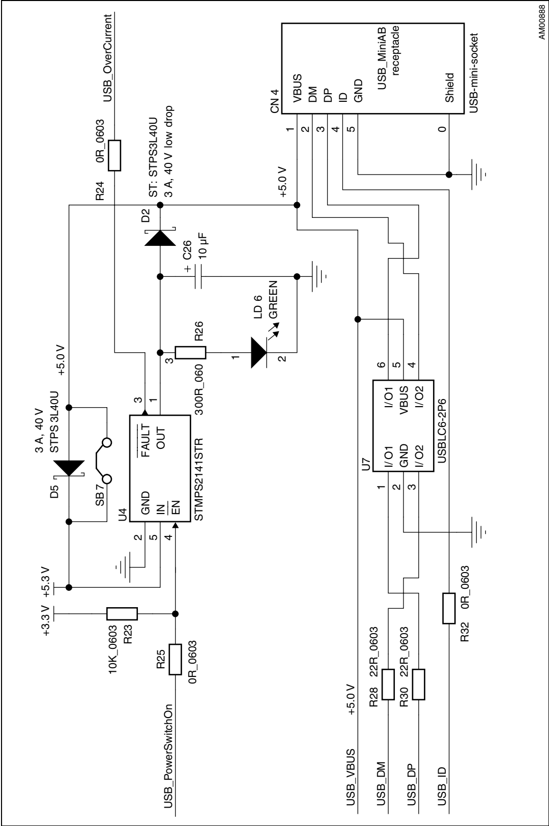
Figure 21. USB-OTG
