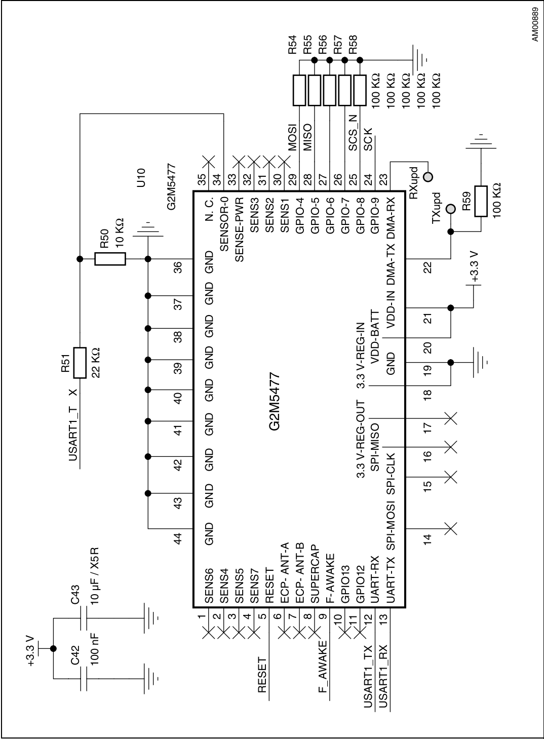
Figure 22. Wi-Fi module-1
