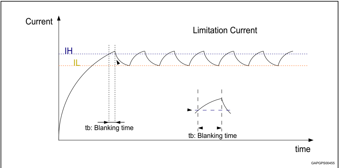
Figure 11. Current limitation
