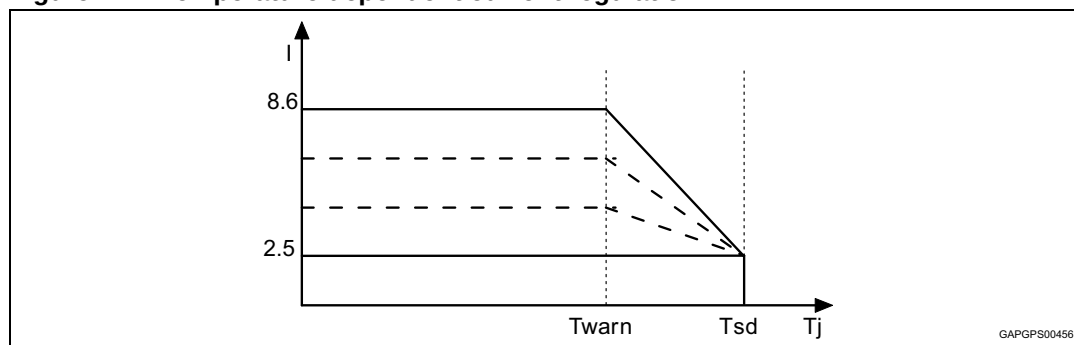
Figure 12. Temperature dependent current regulation
