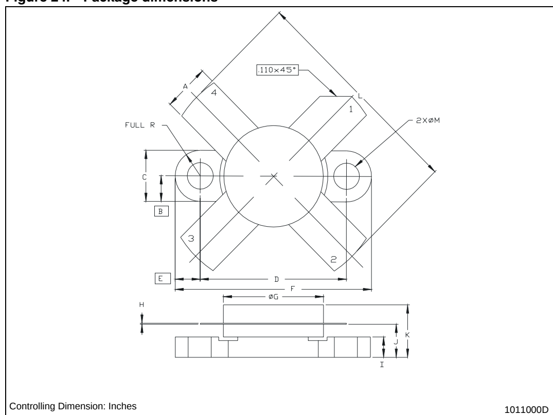
Figure 24. Package dimensions
