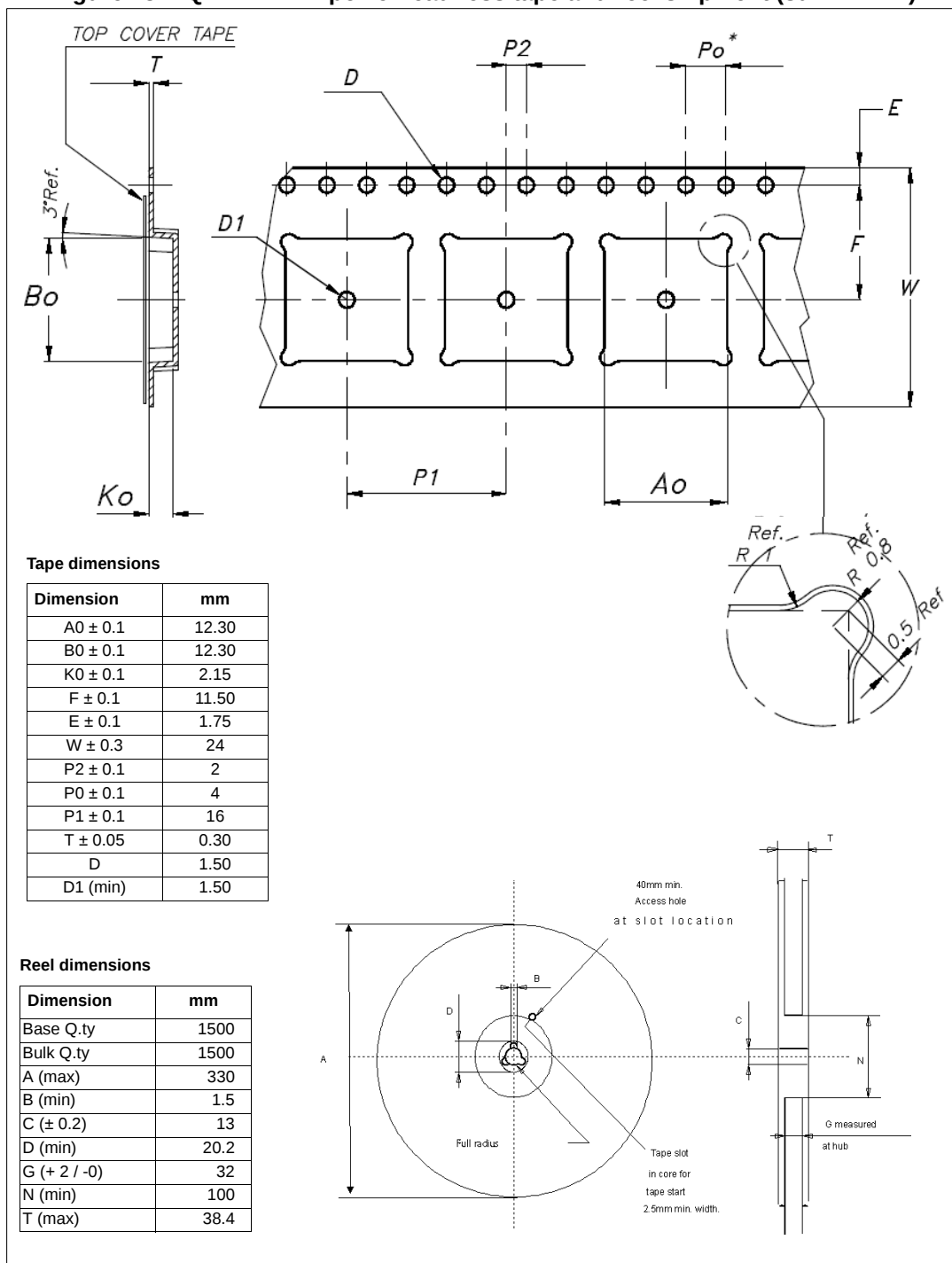
Figure 48. PQFN - 12x12 power lead-less tape and reel shipment (suffix "TR")
