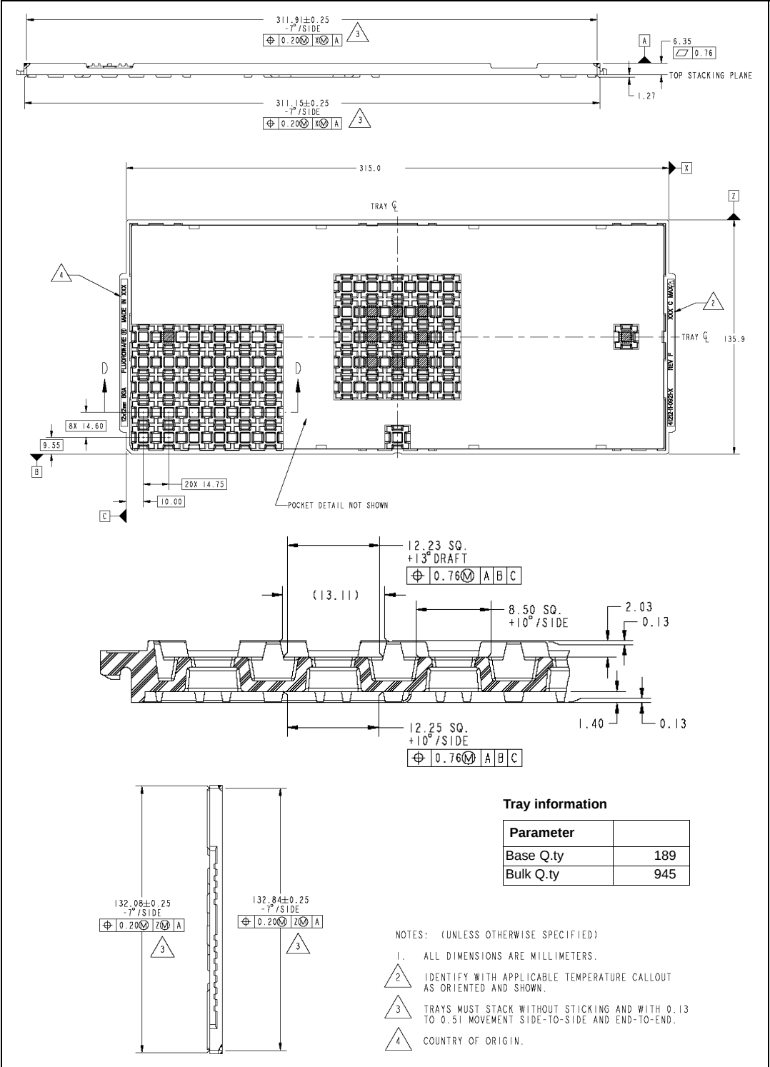
Figure 47. PQFN - 12x12 power lead-less tray shipment (no suffix)
