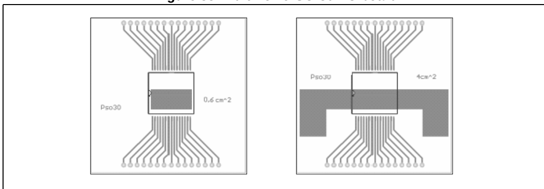
Figure 35. MultiPowerSO-30 PC board
