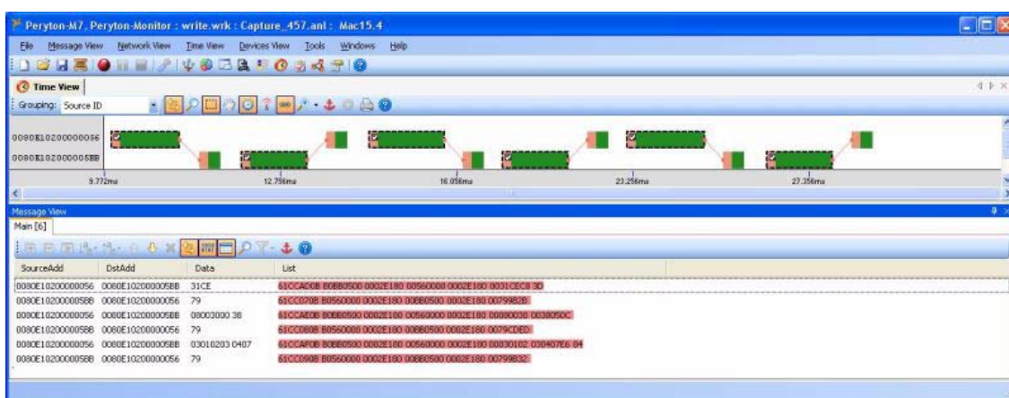
Figure 24. WRITE MEMORY packet example
