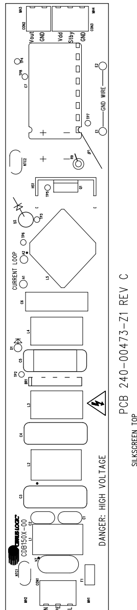
Figure 2. Top Silkscreen
