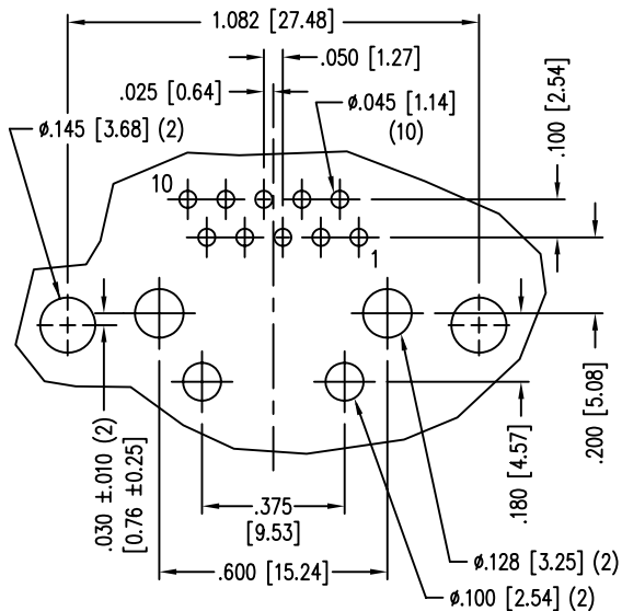
PC BOARD TOP VIEW
