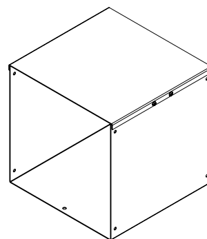
ISOMETRIC VIEW
