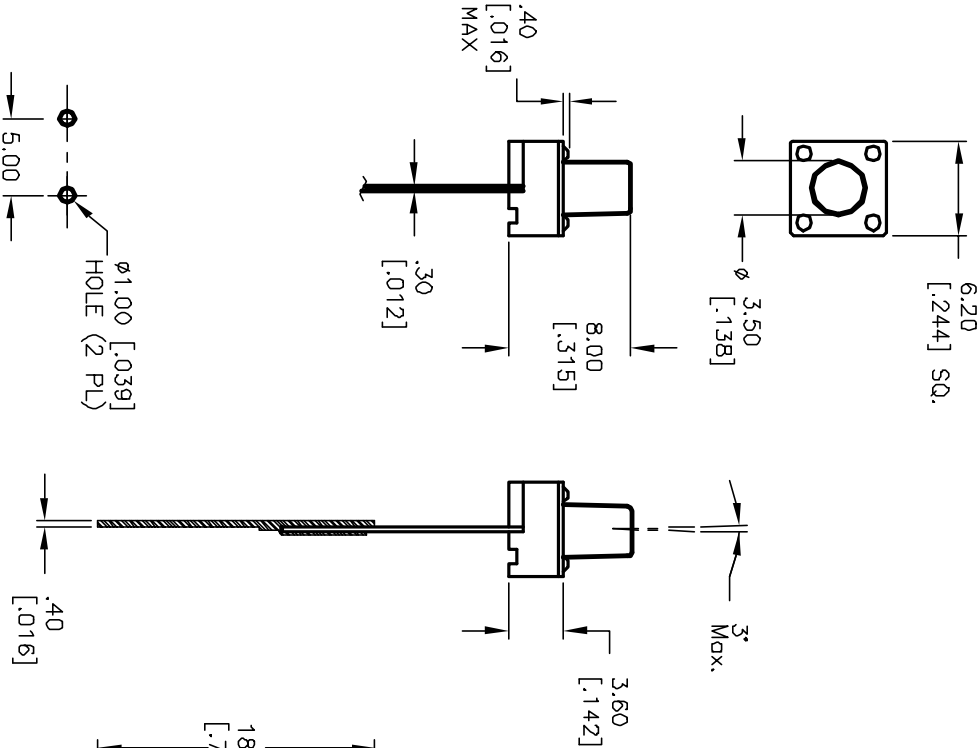
CIRCUIT: SPST
