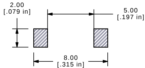
RECOMMENDED P.C.B. LAND SCALE: 4:1
