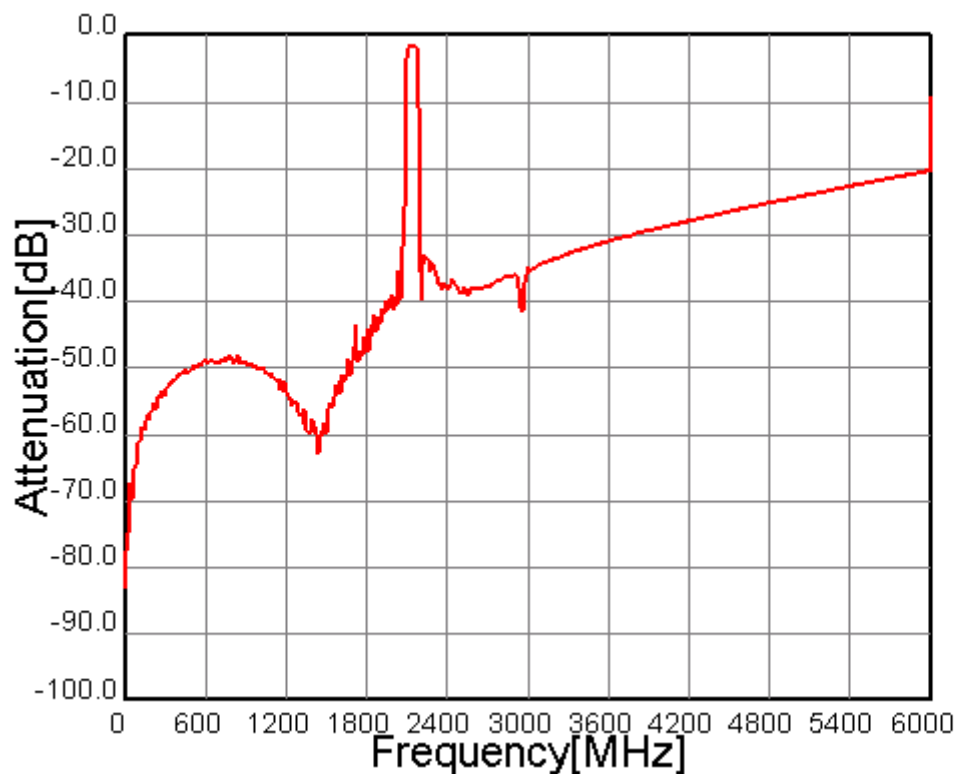
Fig.4 Wide-band Characteristic
