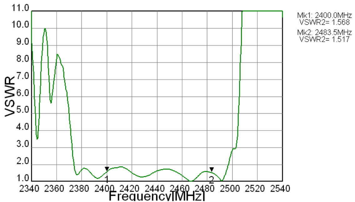
Figure 4. VSWR (Output)
