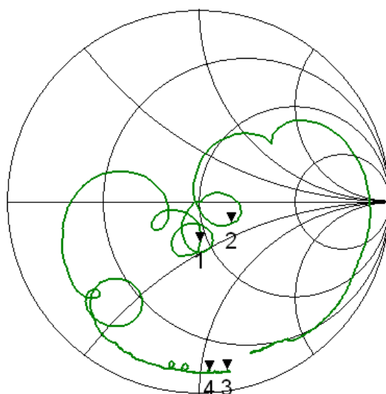
Fig.6 Output Impedance
